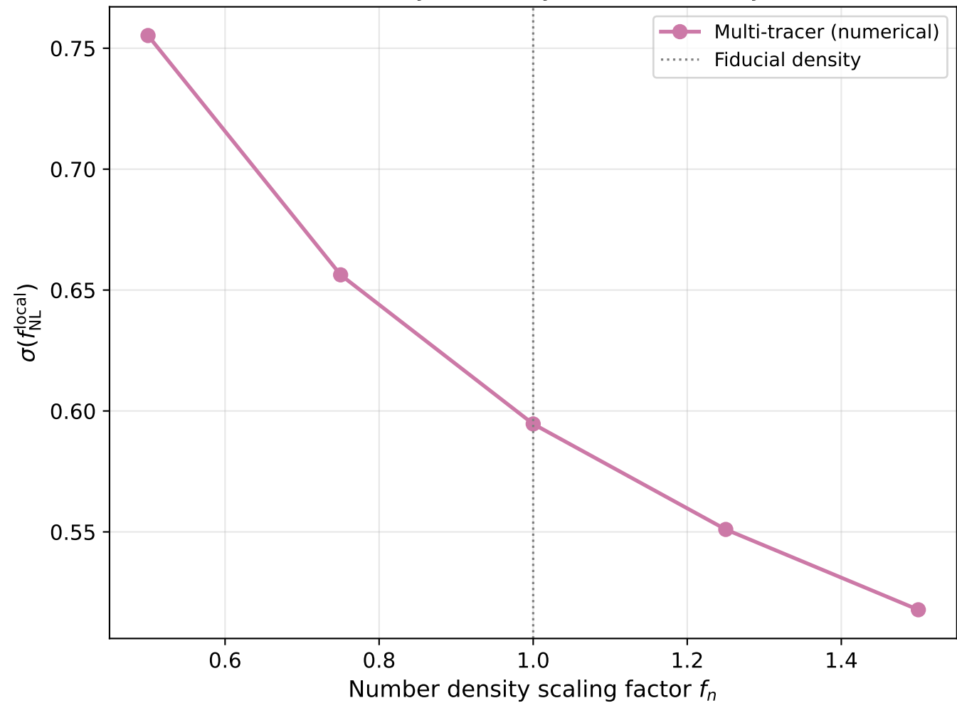
Sensitivity to Galaxy Number Density
