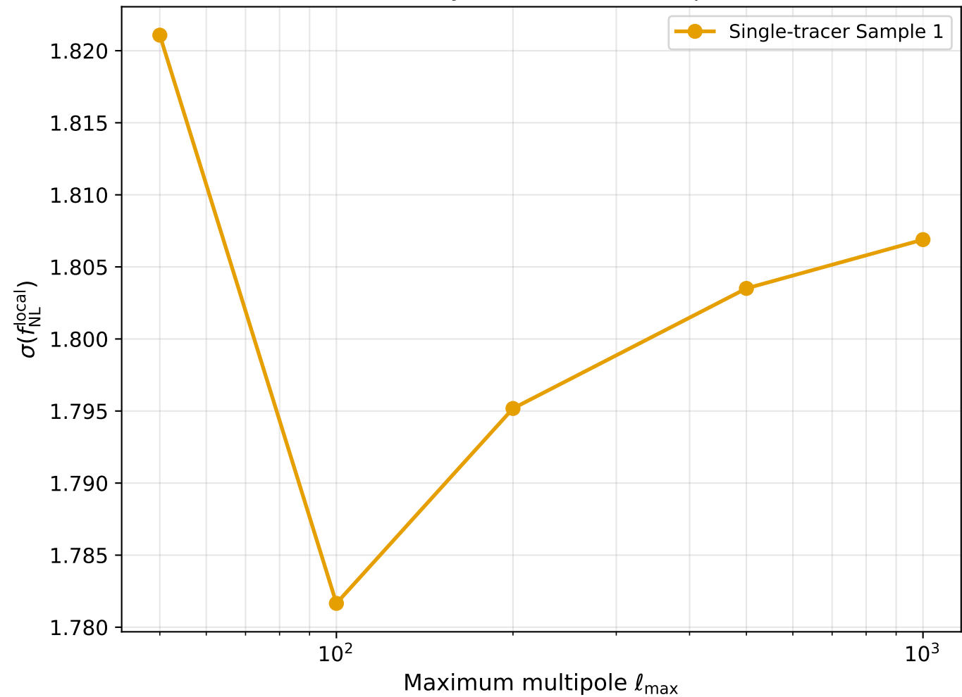
Sensitivity to Maximum Multipole
