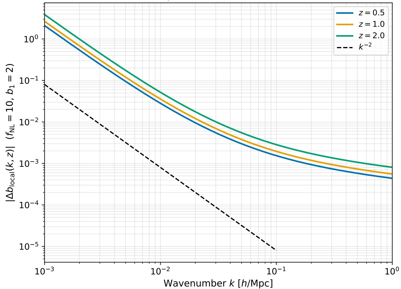
Scale-Dependent Bias from Local PNG
