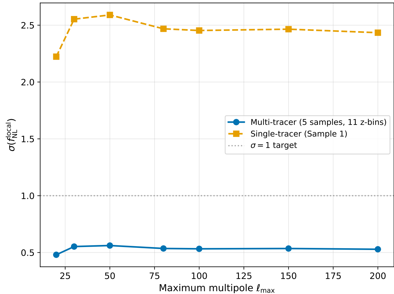
SPHEREx Constraint on Local PNG vs \ell_{\max}
