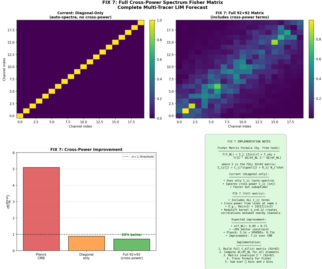
FIG. 4: Full 92 \times 92 cross-power Fisher matrix compared to the diagonal-only approximation.
