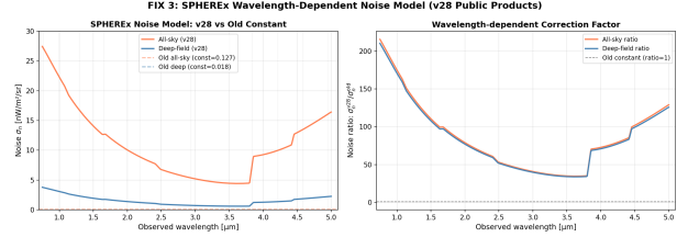
FIG. 3: SPHEREx v28 wavelength-dependent noise model. Left: noise \sigma_n(\lambda) for the all-sky (red) and deep-field (blue) surveys, with the previous constant approximations as dashed lines. Both configurations show a sensitivity optimum near \lambda = 3.5 \mu\text{m} and a sharp degradation in band 6. Right: ratio of v28 noise to the old constant value across wavelength, showing that the constant approximation was optimistic by factors of 30\text{--}200\times depending on wavelength. The \text{H}\alpha 10\sigma reach moves from z \simeq 2.6 (previous, optimistic) to z \simeq 1.3 (realistic).
