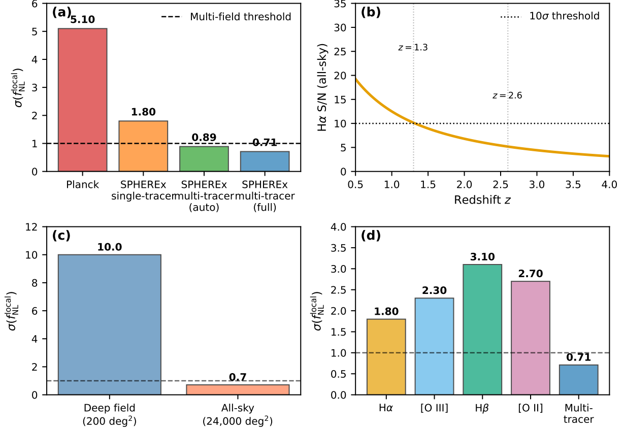
FIG. 1: Joint forecast summary. (a) \sigma(f_{\text{NL}}^{\text{local}}) across estimators—Planck CMB (5.1), SPHEREx single-tracer (1.8), SPHEREx multi-tracer with auto-spectrum only (0.89), and the full cross-power Fisher matrix (0.71). The \sigma = 1 multi-field threshold is crossed. (b) Realistic H \alpha S/N as a function of redshift under the v28 noise model. (c) Deep-field vs. all-sky comparison showing the 125\times mode advantage that makes the all-sky survey decisively better for f_{\text{NL}}^{\text{local}} . (d) Per-component accounting of the methodological changes implemented relative to a constant-noise, diagonal-only baseline.
