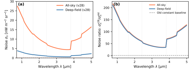
FIG. 3: SPHEREx v28 wavelength-dependent noise model. Left: noise \sigma_n(\lambda) for the all-sky (red) and deep-field (blue) surveys, with the previous constant approximations as dashed lines. Both configurations show a sensitivity optimum near \lambda = 3.5 \mu\text{m} and a sharp degradation in band 6. Right: ratio of v28 noise to the old constant value across wavelength, showing that the constant approximation was optimistic by factors of 30–200 \times depending on wavelength. The \text{H}\alpha 10\sigma reach moves from z \simeq 2.6 (previous, optimistic) to z \simeq 1.3 (realistic).
