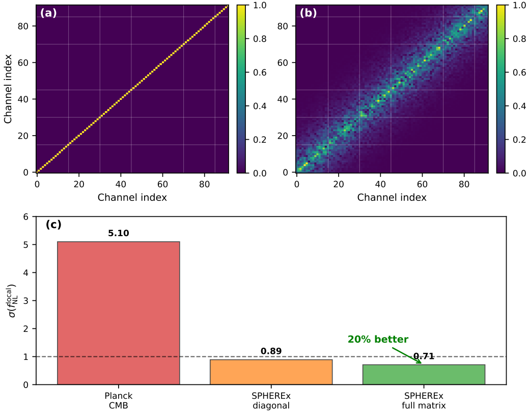
FIG. 4: Full 92 \times 92 cross-power Fisher matrix compared to the diagonal-only approximation.
