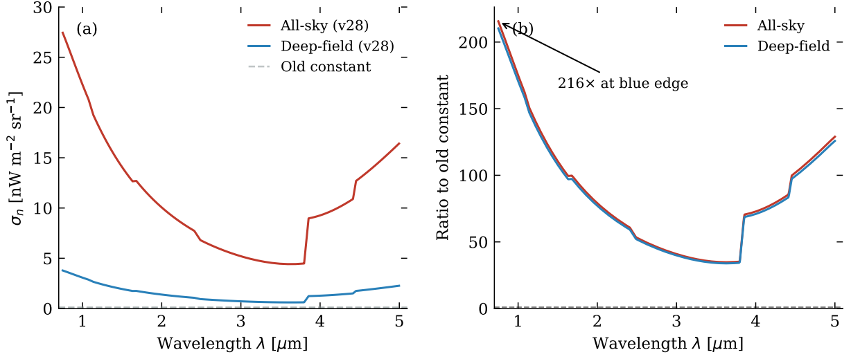
FIG. 3: SPHEREx v28 wavelength-dependent noise model. Left: noise \sigma_n(\lambda) for the all-sky (red) and deep-field (blue) surveys, with the previous constant approximations as dashed lines, with band boundaries marked. Both configurations show a sensitivity optimum near \lambda = 3.5 \mu\text{m} and a sharp degradation in band 6. Right: ratio of v28 noise to the old constant value across wavelength, showing that the constant approximation was optimistic by factors of 30–200 \times depending on wavelength. The \text{H}\alpha 10\sigma reach moves from z \simeq 2.6 (previous, optimistic) to z \simeq 1.3 (realistic). Vertical dotted lines mark the six SPHEREx band boundaries.
