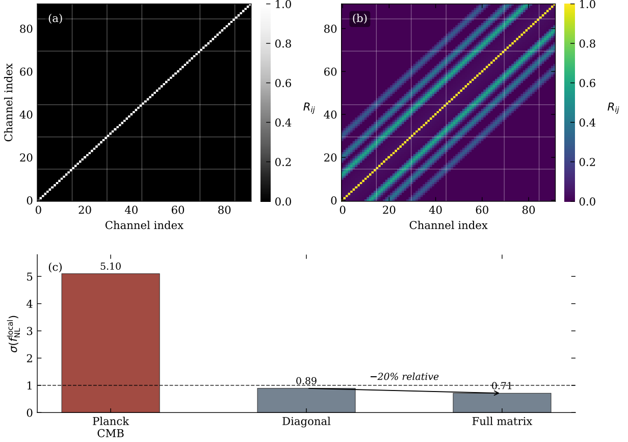
FIG. 4: Full 92 \times 92 cross-power Fisher matrix compared to the diagonal-only approximation. Top: correlation matrix R_{ij} = \Sigma_{ij} / \sqrt{\Sigma_{ii}\Sigma_{jj}} at a representative multipole \ell \approx 75 —diagonal-only (left) shows only auto-correlations, while the full matrix (right) shows concentrated off-diagonal weight at line pairs observed at matched physical redshifts (visible as bright streaks parallel to the diagonal). Bottom: the resulting \sigma(f_{\text{NL}}^{\text{local}}) improves from 0.89 to 0.71, a 20% gain consistent with the Seljak [6] cosmic-variance cancellation.
