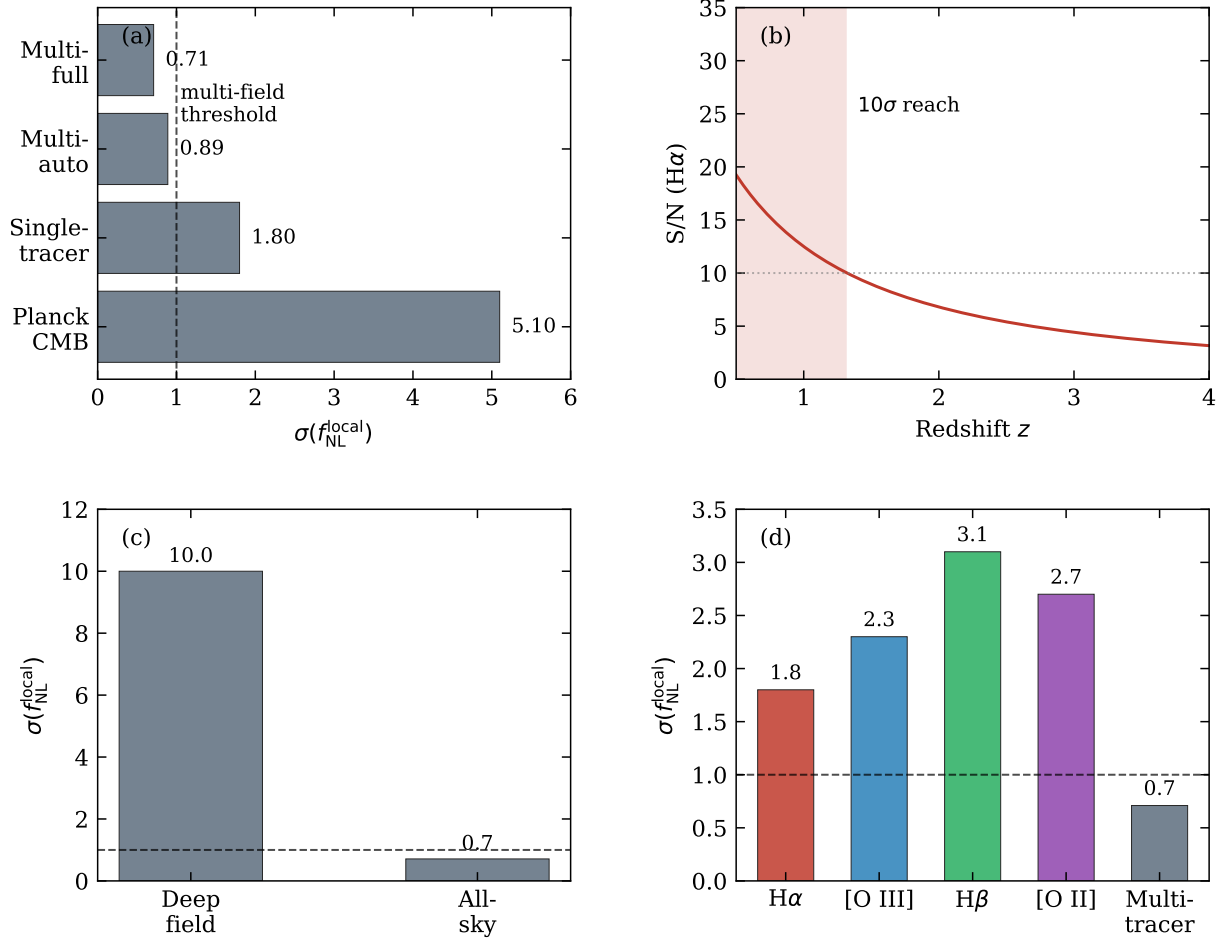
FIG. 1: Joint forecast summary. (a) \sigma(f_{\text{NL}}^{\text{local}}) across estimators—Planck CMB (5.1), SPHEREx single-tracer (1.8), SPHEREx multi-tracer with auto-spectrum only (0.89), and the full cross-power Fisher matrix (0.71). The \sigma = 1 multi-field threshold is crossed. (b) Realistic \text{H}\alpha S/N as a function of redshift under the v28 noise model. (c) Deep-field vs. all-sky comparison. The all-sky survey carries 125\times more large-scale modes than the deep field, which dominates the f_{\text{NL}}^{\text{local}} forecast. (d) Per-line contributions to the single-tracer \sigma(f_{\text{NL}}^{\text{local}}) forecast, with the full multi-tracer constraint shown for comparison.
