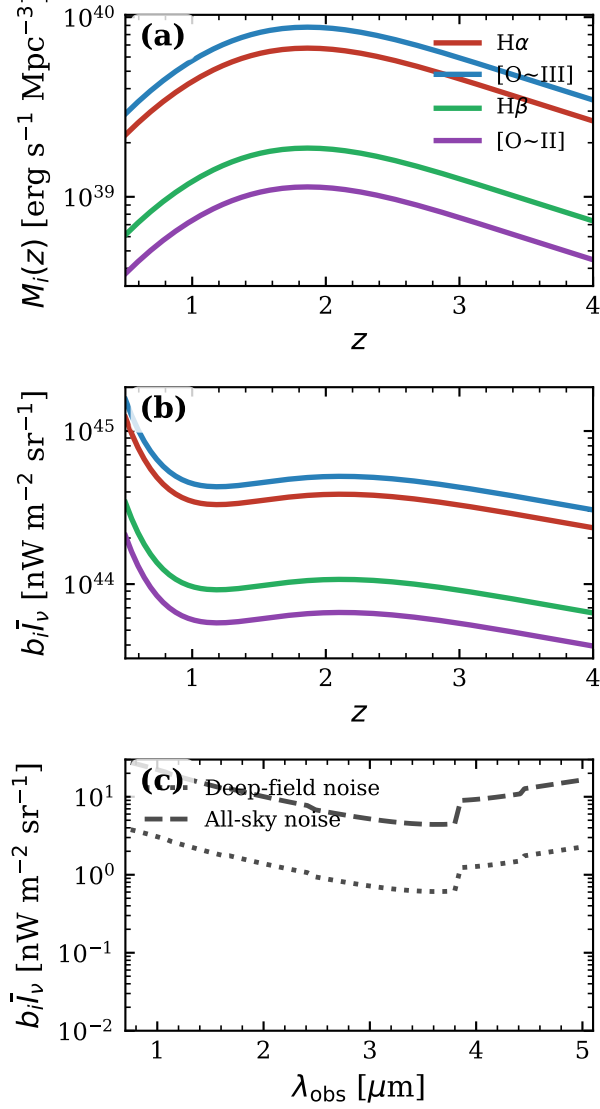
FIG. 2: Bias-weighted intensity for the four SPHEREx emission lines. Top: the comoving line luminosity density M_i(z) , peaking near cosmic noon, z \simeq 2 . Middle: the bias-weighted intensity b_i \bar{I}_\nu^{(i)} as a function of redshift. Bottom: intensity as a function of observed wavelength with the SPHEREx deep-field (dotted) and all-sky (dashed) noise floors overlaid. The bright-line ordering \text{H}\alpha > [\text{O III}] > \text{H}\beta > [\text{O II}] at z = 2 holds only after the [\text{O II}] dust attenuation is corrected to
