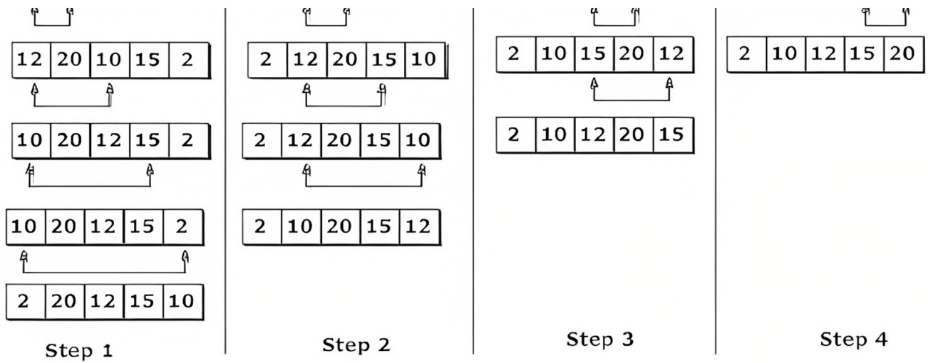
Figure: Selection Sort
