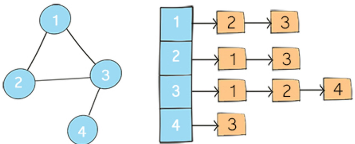
undirected graph and its adjacency list
