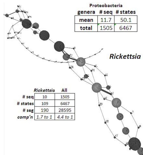
Fig. 4. EMM visualization showing compression of sequences. EMM achieves sequence compression by clustering similar segments of sequences into nodes. EMM for genus Rickettsia is shown to compress 190 sequence segments of 80 nucleotides into 109 nodes of nsf with a numerical vector of size 64. Likewise, all genera models are compressed achieving a ratio of 4.4 to 1 space efficiency.
