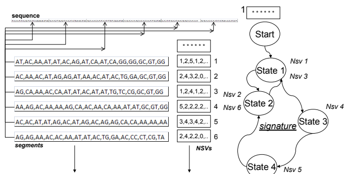
Fig. 1. The Model Building Process. Numerical Summary Vectors (NSV) constitute the numerical representations of equal sized segments along a 16S sequence which are used in building an EMM signature. Signature building starts with a start state; as each NSV is processed, it is compared to the existing states of the model. If the NSV is not found to be close enough (per a Squared Euclidean threshold) as in the case of NSV 1, a new state (1) is created with the new NSV as its first cluster member; otherwise, the new NSV (as in the case of NSV 3) is simply added to the matching cluster state node (state 1). When all NSVs are processed, the model building process is finished.
