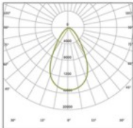
H00215 (100W/60°) H00218 (150W/60°) H00221 (200&240W/60°)
