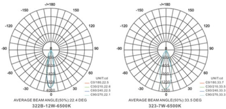
LIGHT DISTRIBUTION CURVE
