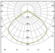
H00213 (100W/115°) H00216 (150W/115°) H00219 (200&240W/115°)
