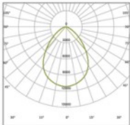
H00214 (100W/85°) H00217 (150W/85°) H00220 (200&240W/85°)
