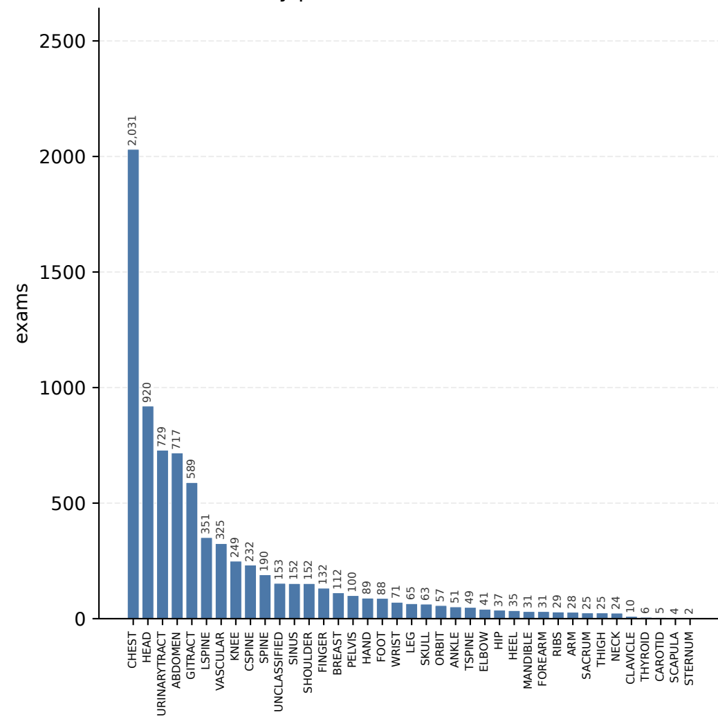
Body part (derived), train subset
