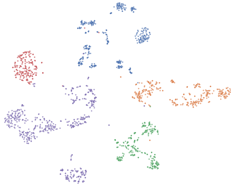
BiomedCLIP, fine-tuned
