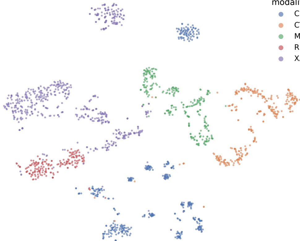
BiomedCLIP, zero-shot
