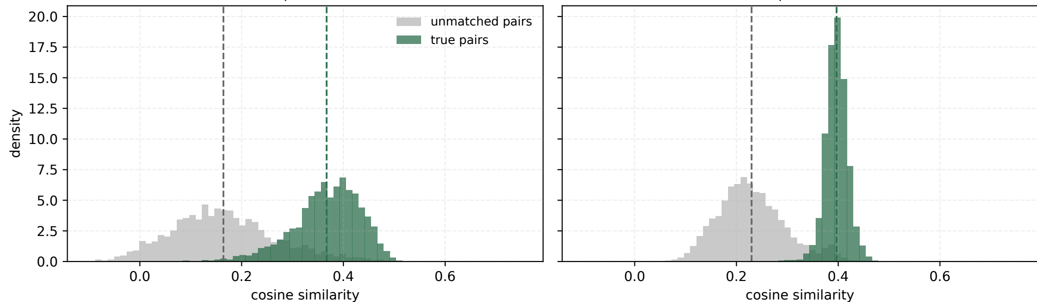
BiomedCLIP, zero-shot mean separation 0.203
