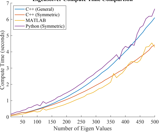
Eigensolver Compute Time Comparison
