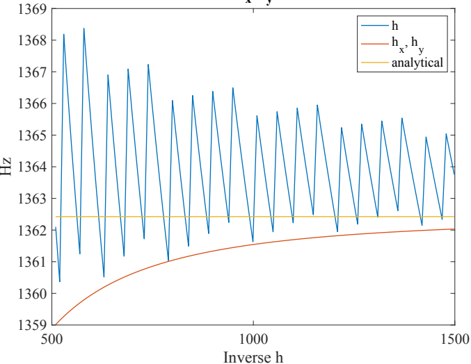
Mode 5: h vs h_x, h_y vs analytical
