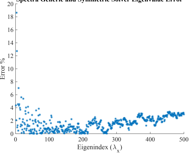
Spectra Generic and Symmetric Solver Eigenvalue Error
