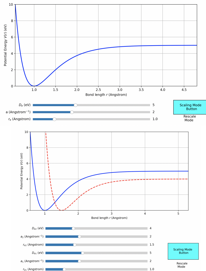
Figure S16: (Top) Morse potential curve for a single bond and (Bottom) Morse potential curves for a pair of different bonds.
