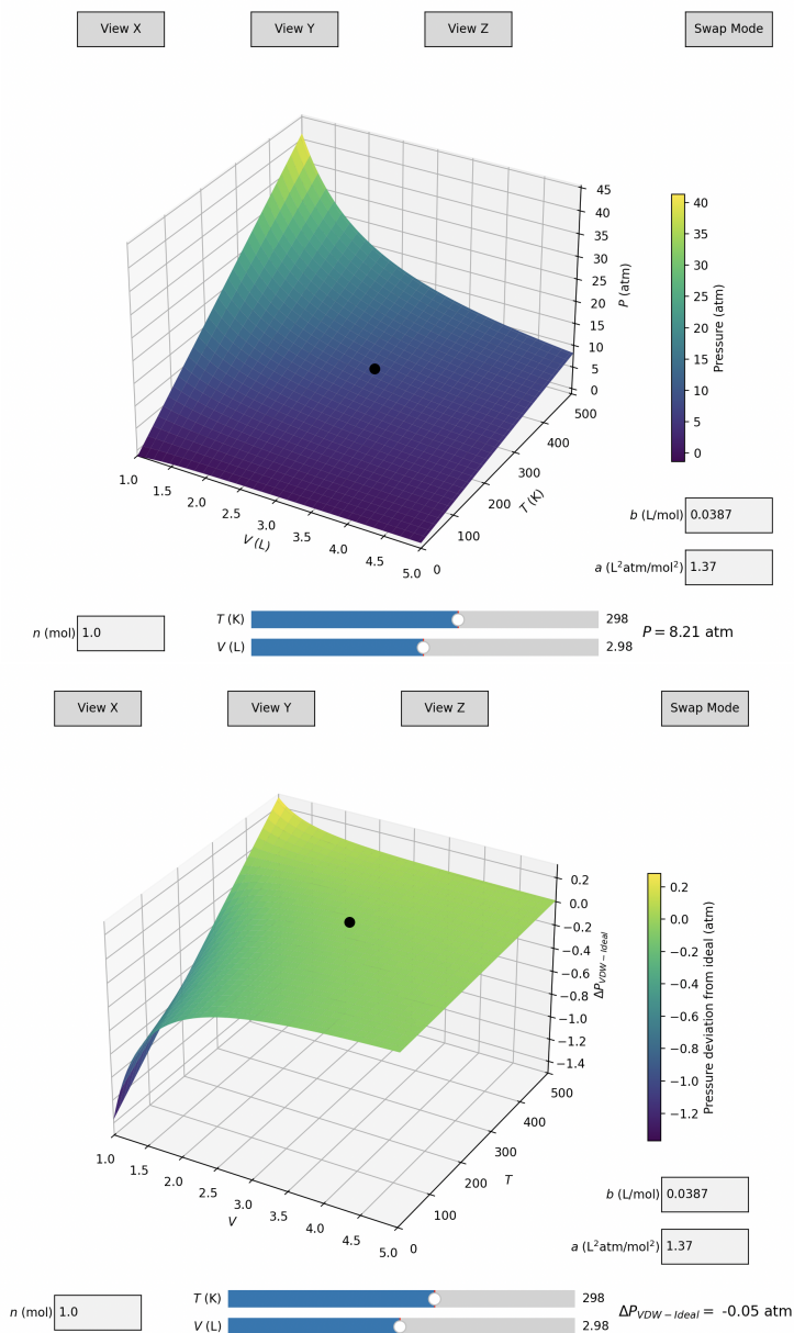
Figure S14: (Top) Example of the surface plot generated for a Van Der Waals gas and (bottom) the deviation of the gas pressure from the corresponding ideal gas.
