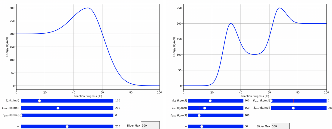
Figure S7: Examples of single and two step uncatalyzed exoergic (left) and endoergic (right) reaction energy profiles.
