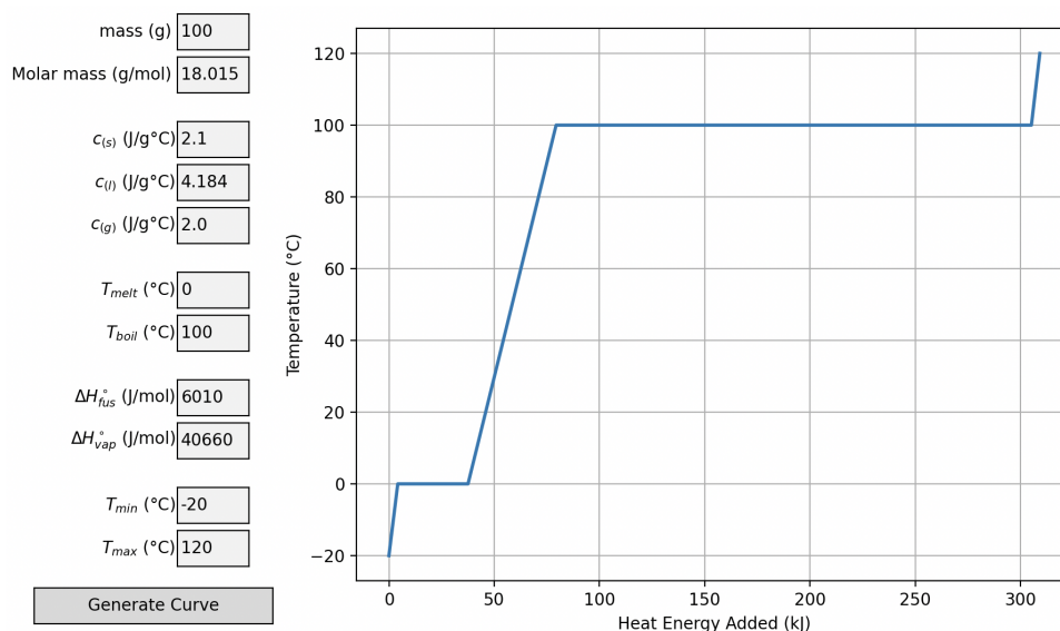
Figure S4: Example of a heating curve for water.
