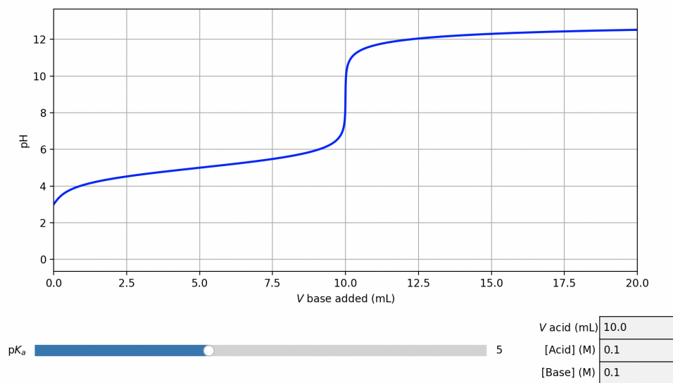
Figure S10: Example of a monoprotic titration curve generated with the Python module.
