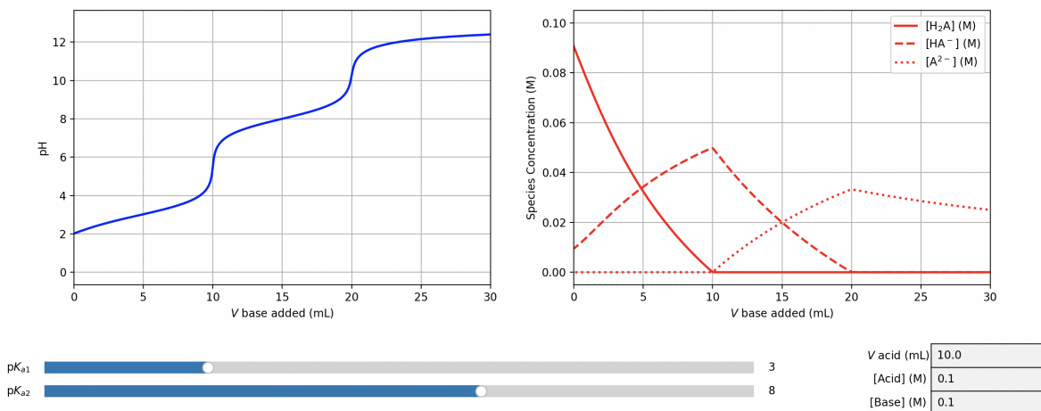
Figure S11: Example of the speciation curves (right) for a diprotic acid titration curve (left).
