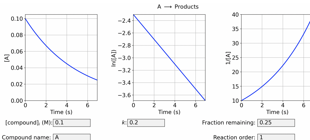
Figure S6: Examples of plots that can be compared to the linearized integrated rate laws to determine reaction order.
