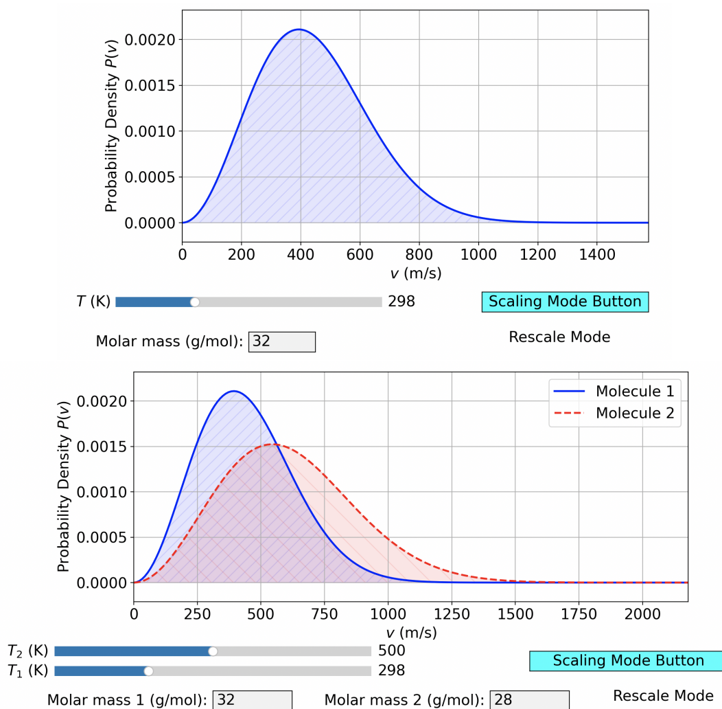
Figure S15: (Top) Maxwell-Boltzmann distribution for a single gas and (Bottom) Maxwell-Boltzmann distributions for a pair of gases.
