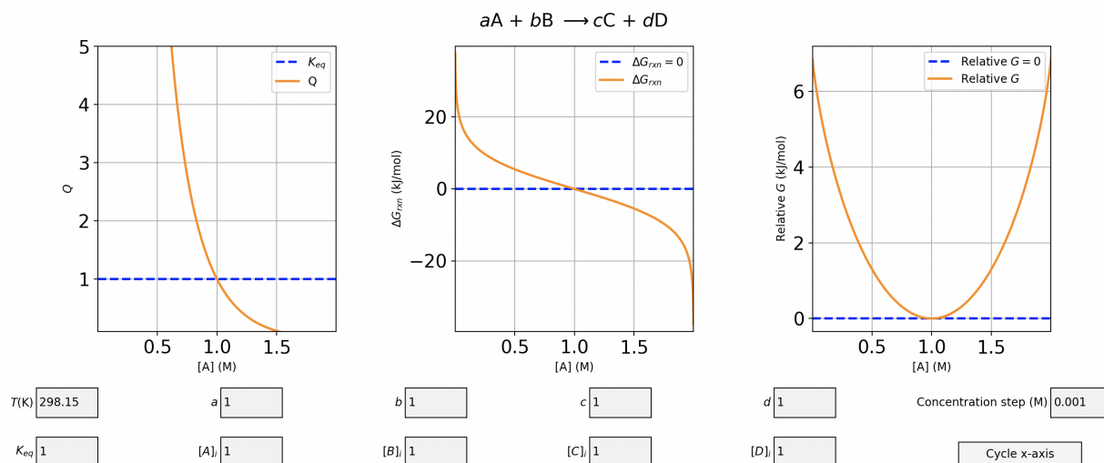
Figure S9: Example of the Gibbs free energy and reaction quotient plots for a particular two reactant and two product reaction.
