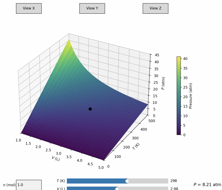
Figure S13: Example of the surface plot generated for an ideal gas.
