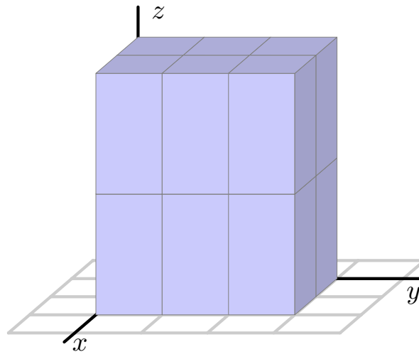
Figure 11.7.1 A partitioned three-dimensional domain.
