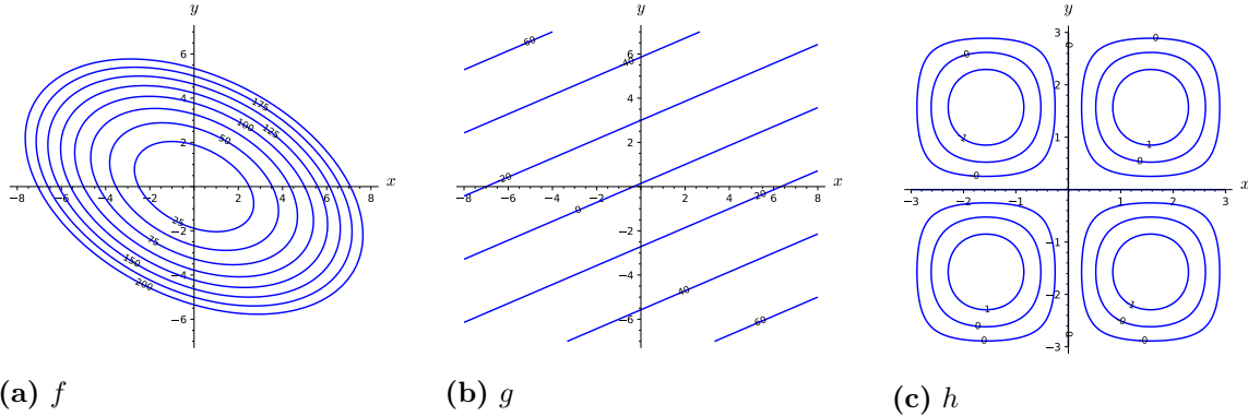
Figure 12.1.7 Three sets of level curves
