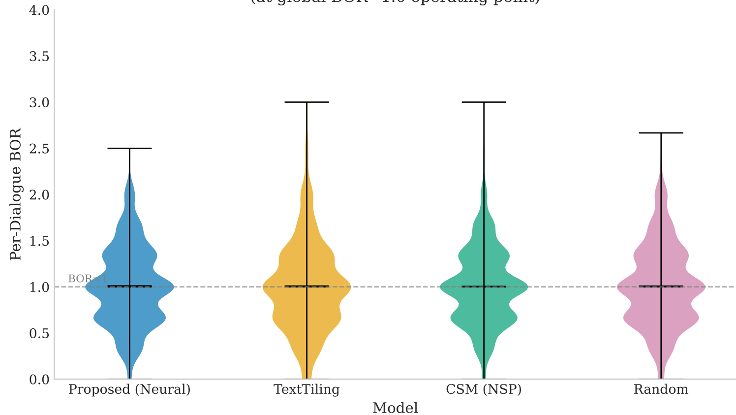
DialSeg711: Per-Dialogue BOR Distribution (at global BOR \approx 1.0 operating point)
