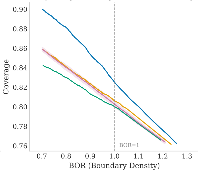
SuperSeg: Coverage Near Gold Density
