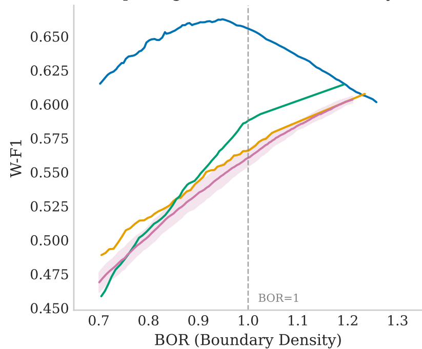
SuperSeg: W-F1 Near Gold Density
