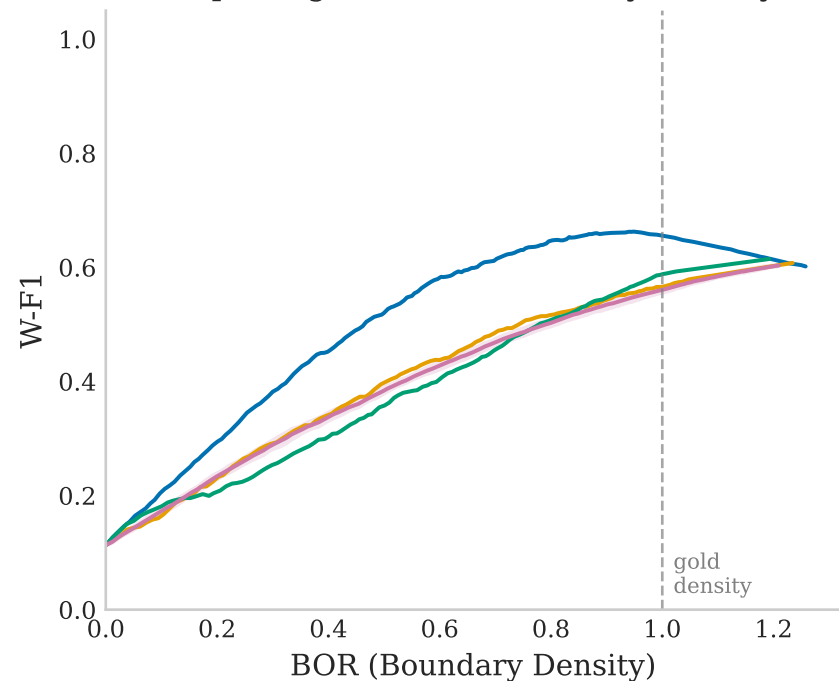
SuperSeg: W-F1 vs Boundary Density
