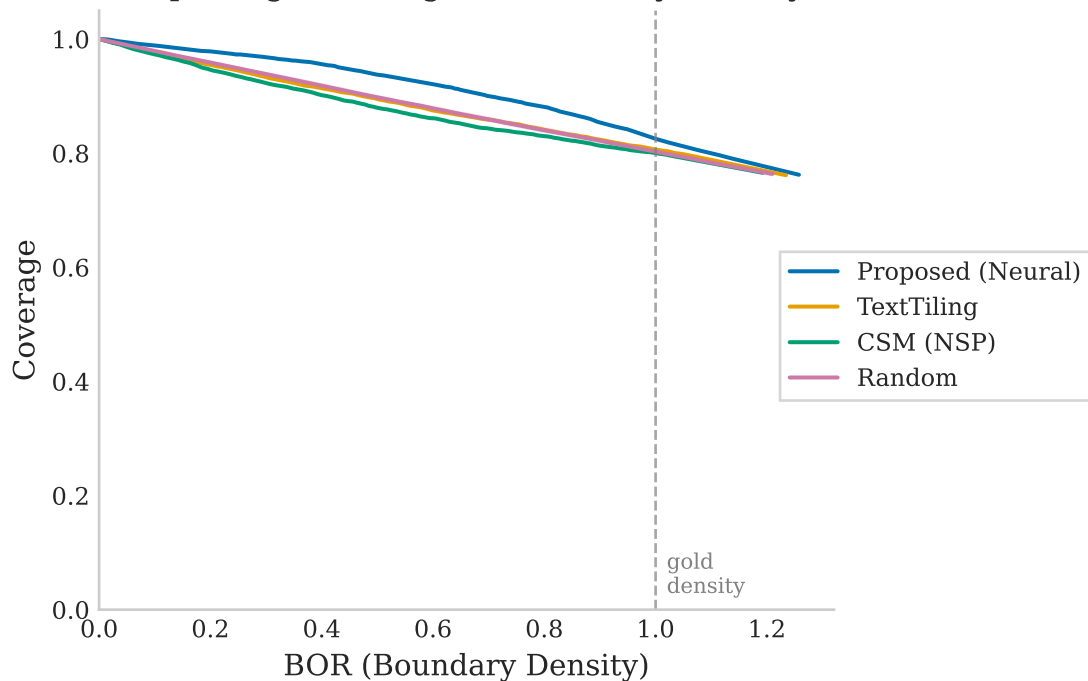
SuperSeg: Coverage vs Boundary Density
