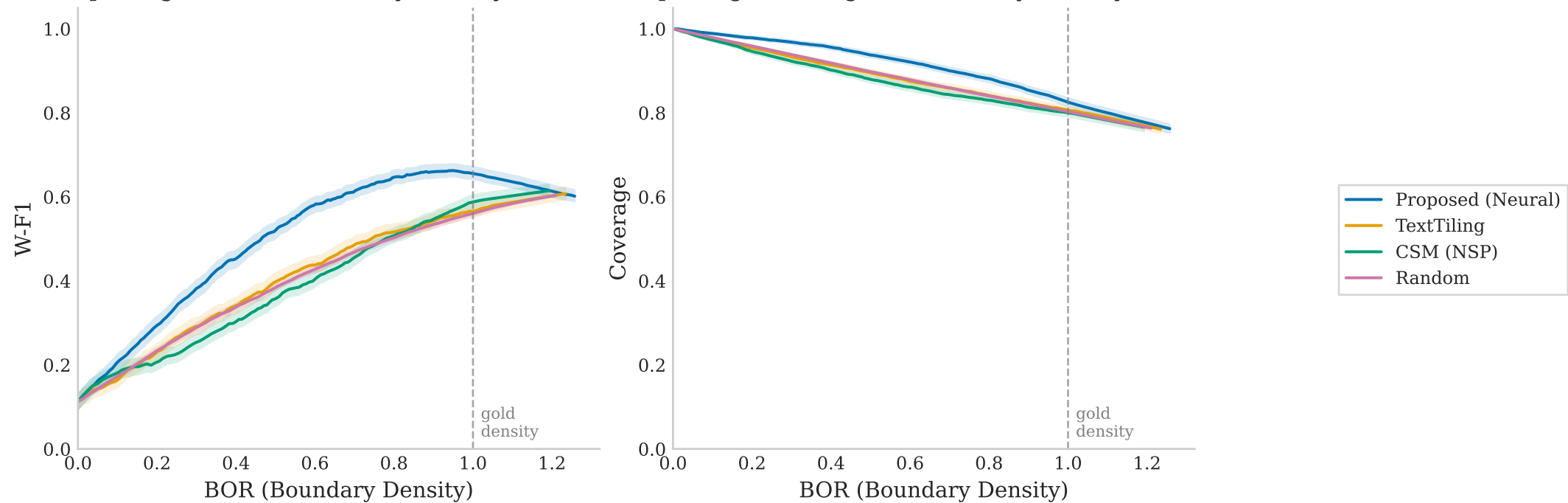
SuperSeg: W-F1 vs Boundary Density (95% CI) SuperSeg: Coverage vs Boundary Density (95% CI)
