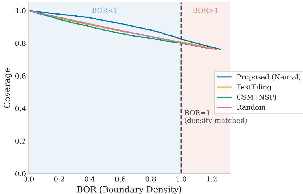
SuperSeg: Coverage vs Boundary Density
