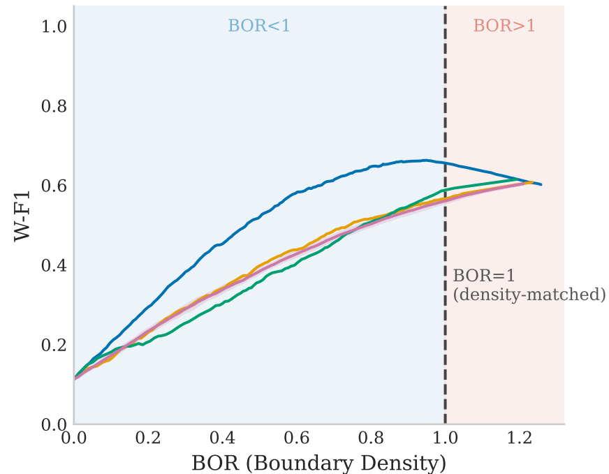
SuperSeg: W-F1 vs Boundary Density
