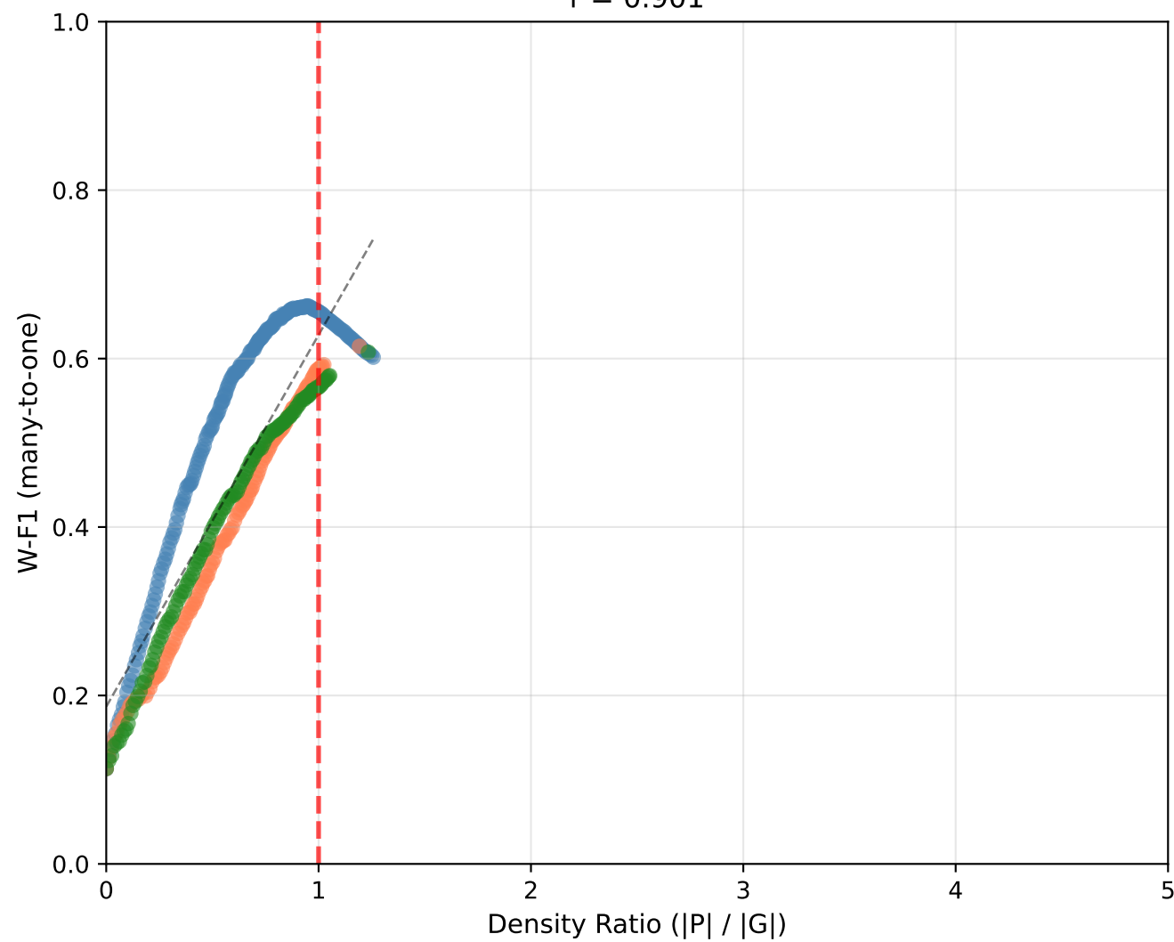
SUPERSEG: W-F1 (many-to-one) r = 0.901
