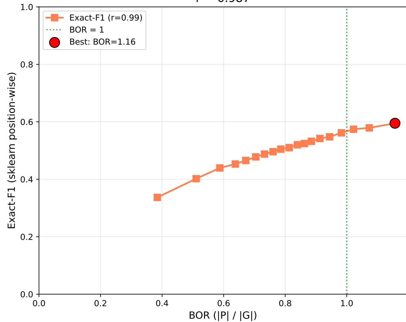
superseg: Exact-F1 vs BOR r = 0.987
