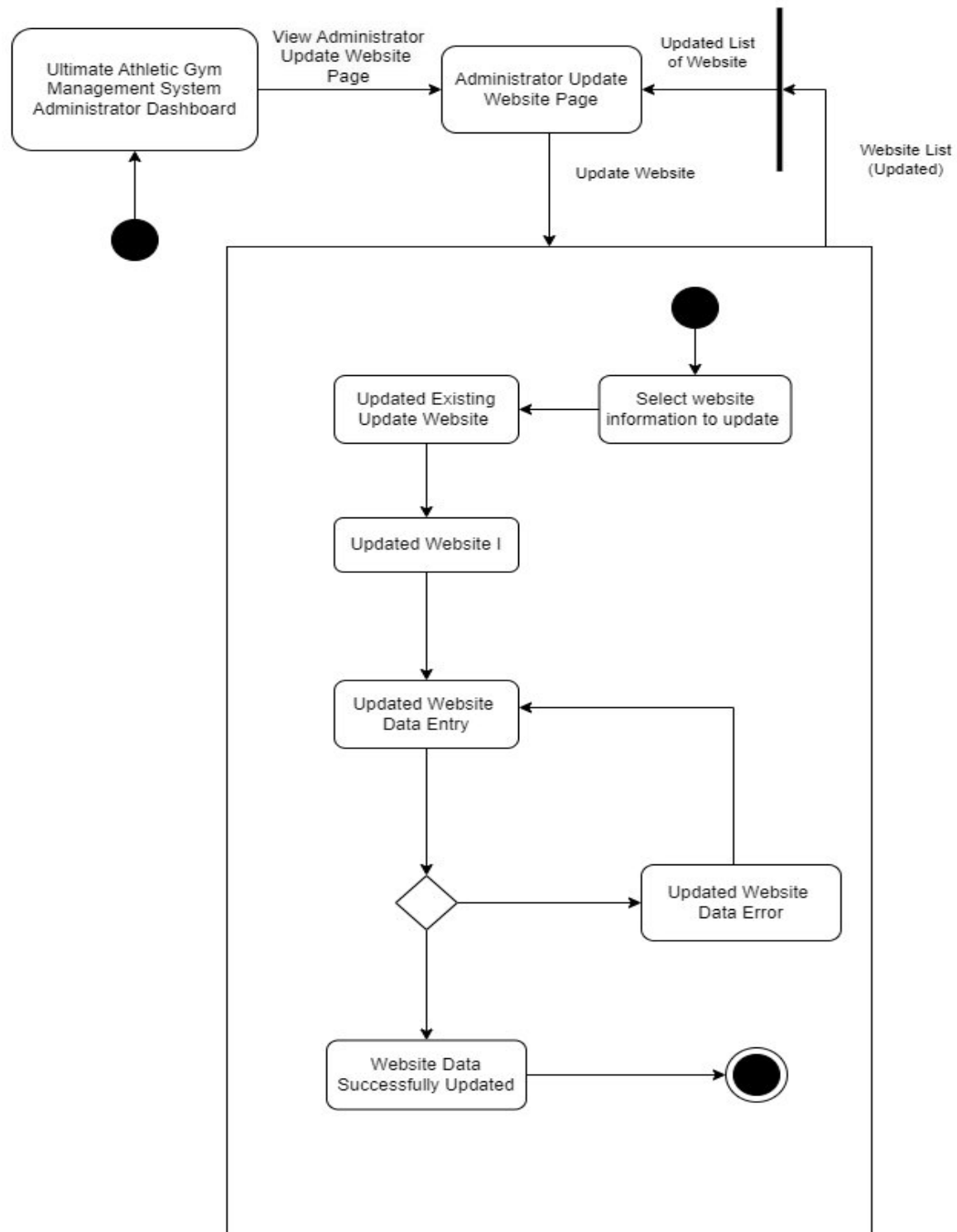
Figure 9: Update Website Information state chart model components
