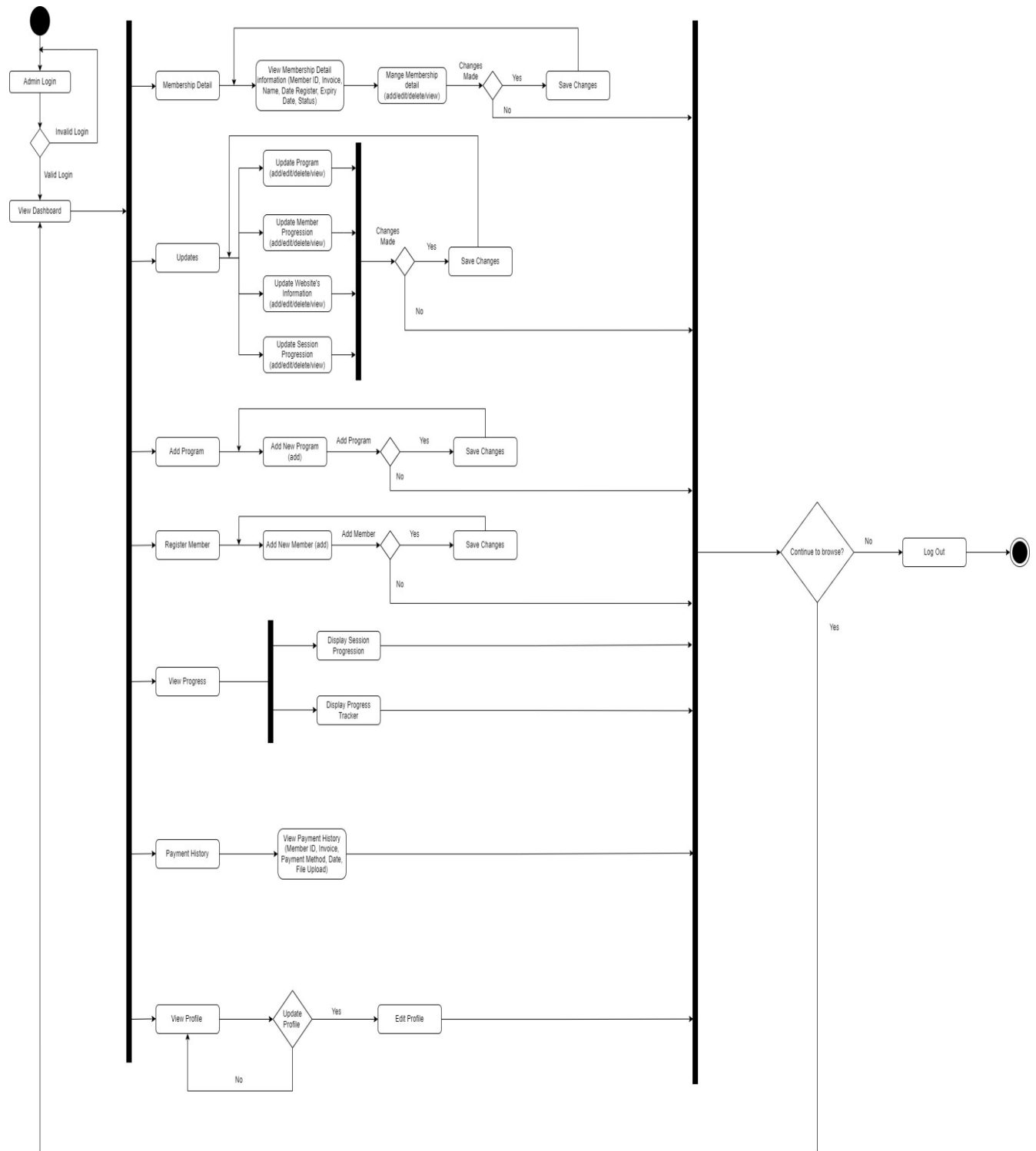
Figure 4: Admin state chart - overall view of Ultimate Athletic Gym Management System using state chart through the administrator link.
