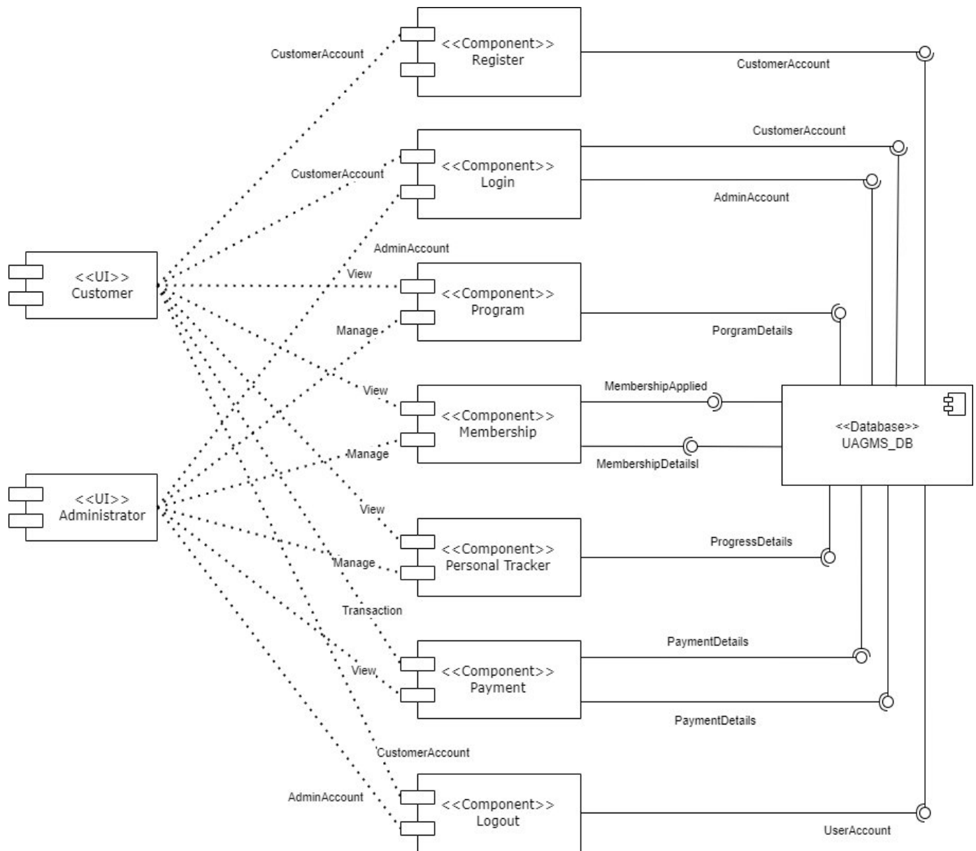
Figure 2: Component Diagram of Ultimate Athletics Gym Management System
