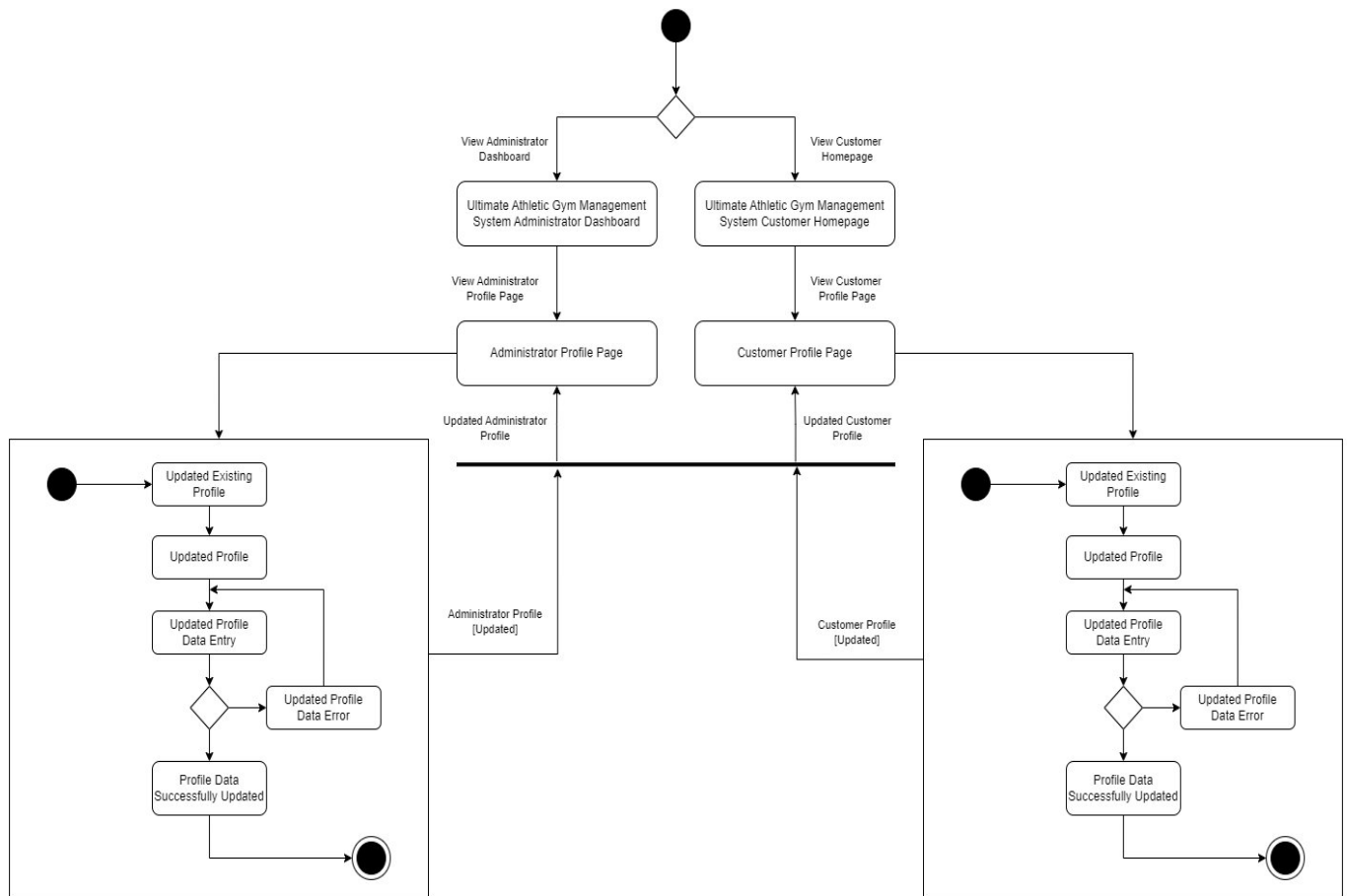
Figure 5: Update Profile state chart model components
