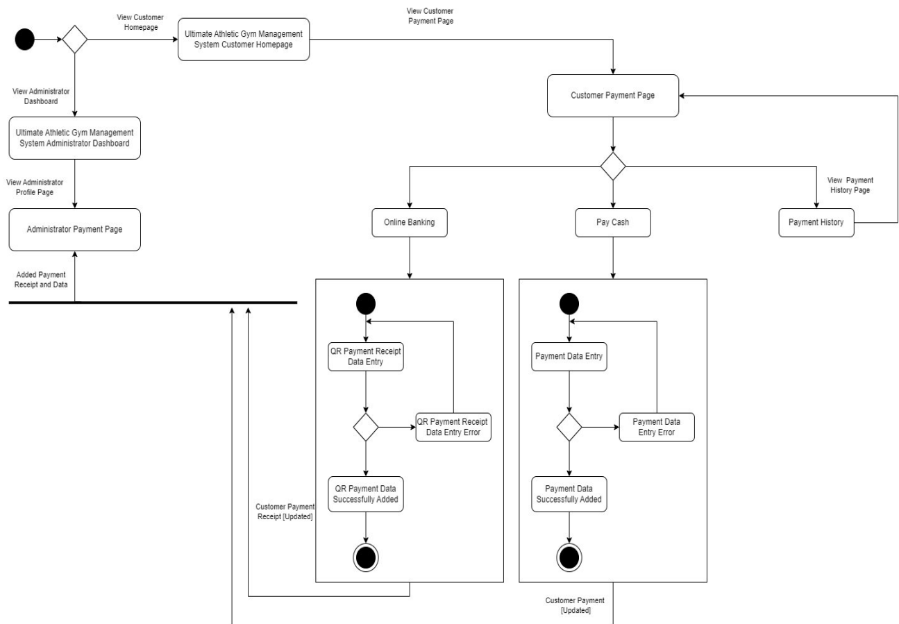
Figure 6: Payment state chart model components
