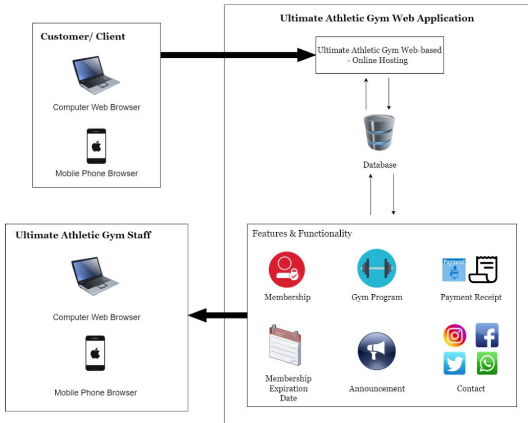
Figure 1: System architecture of Ultimate Athletic Gym Management System
