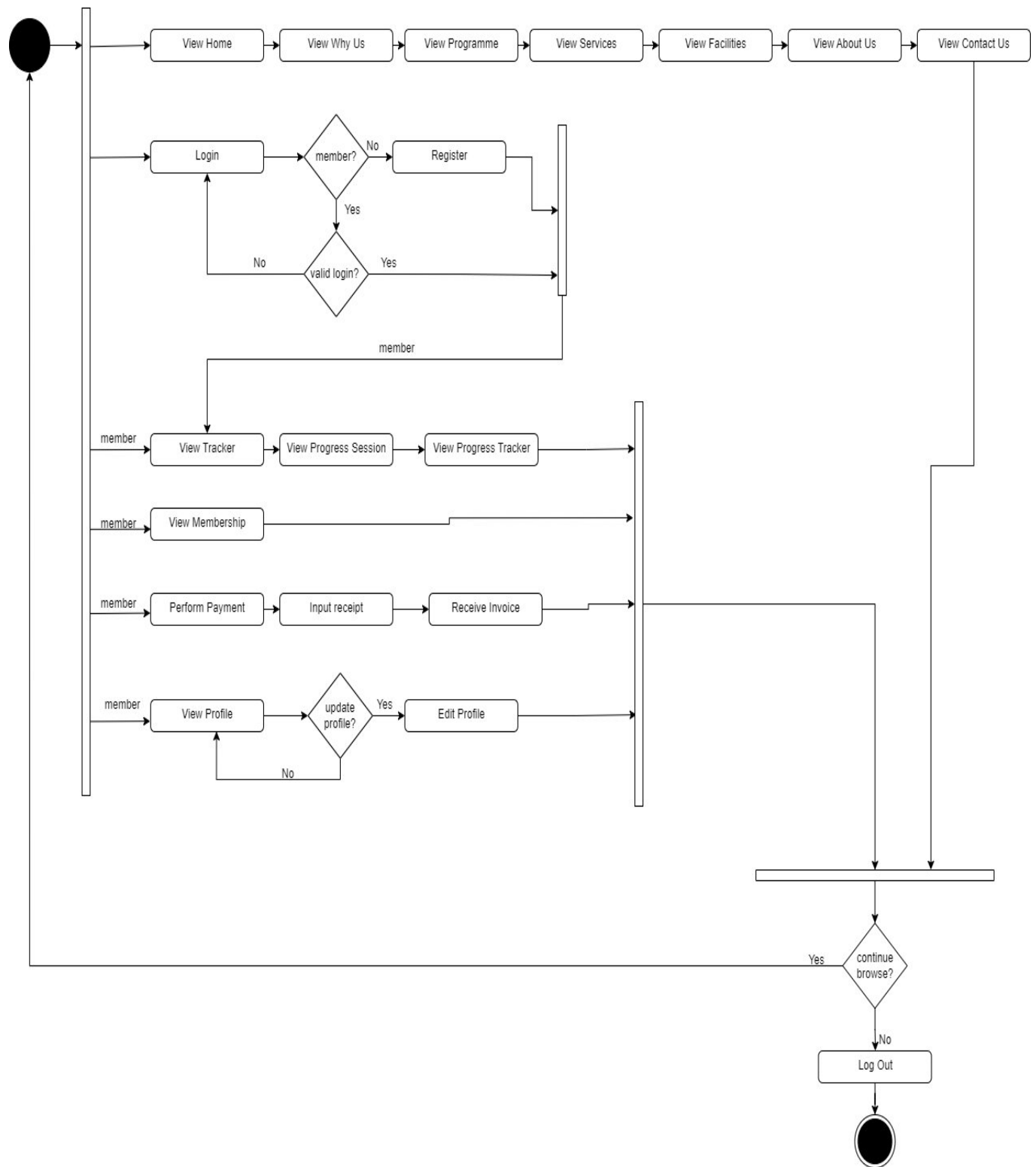
Figure 3: Customer state chart – overall view of Ultimate Athletic Gym Management System using state chart through the customer entity
