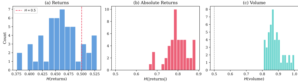
Figure 1: Distribution of full-sample Hurst exponents across 50 S&P 500 constituents (2015–2026). (a) Returns cluster around H = 0.5 . (b) Absolute returns show strong long memory ( H \approx 0.8 ). (c) Volume exhibits the strongest persistence ( H \approx 0.9 ).
