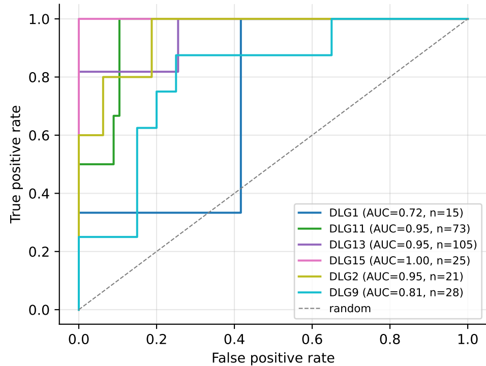
(a) ROC per held-out graph (mean AUC = 0.897)
