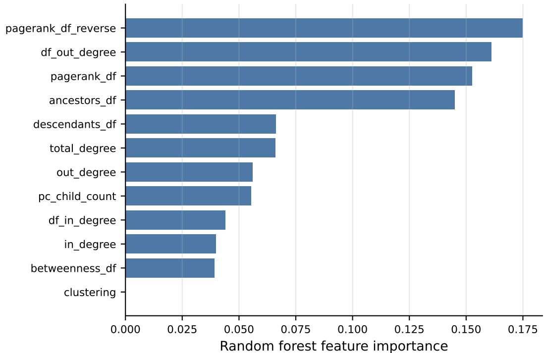
(b) Feature importance (Gini, trained on all 6 graphs)
