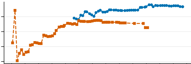
D3 normalized spectral gap
