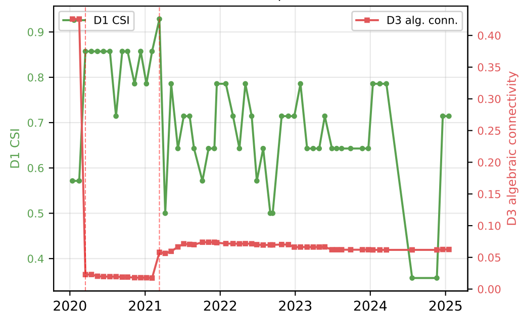
mattermost: descriptor evolution
