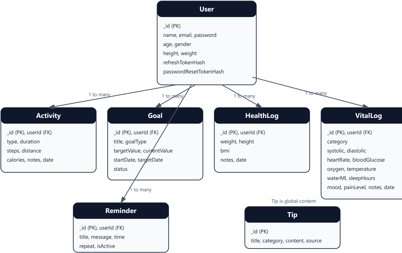
Wellness Hub Database ER Diagram
