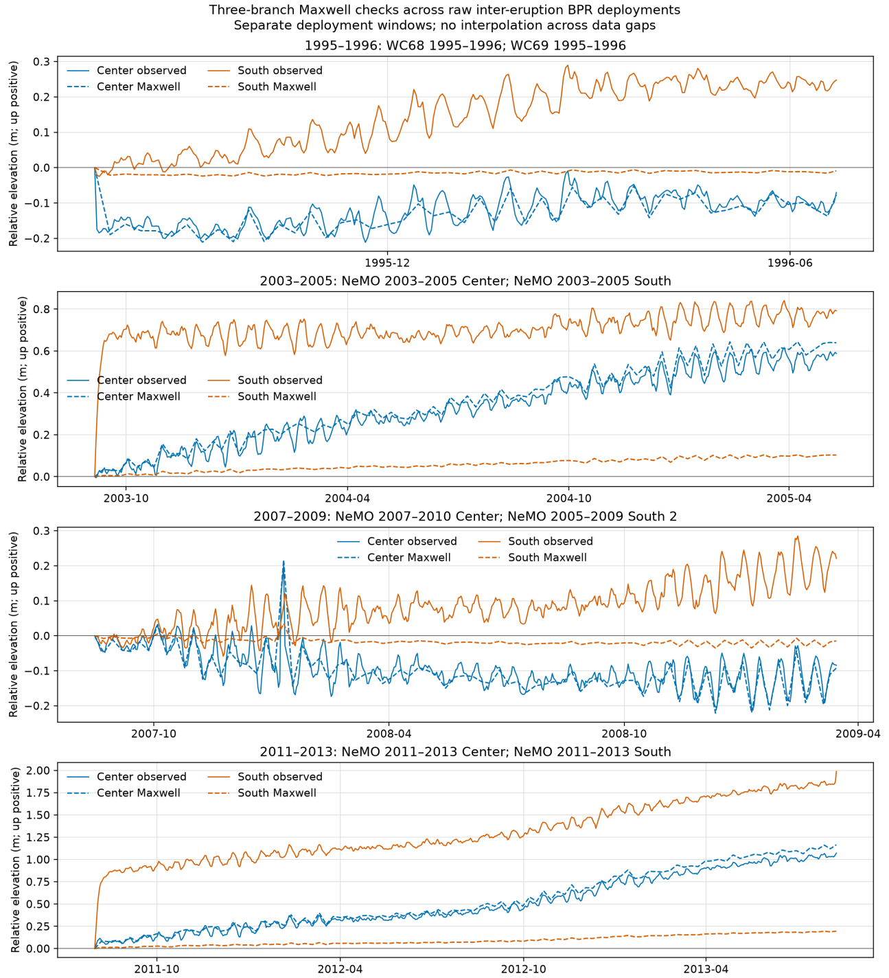
Figure 6: Three-branch Maxwell checks for four raw Center/South deployment overlaps from 1995 through 2013. Each deployment pair is independently zeroed; gaps are not interpolated. Center pressure uses static elastic compliance, and the synthetic branch parameters and uncorrected records are diagnostic assumptions. Generated by make historical-generalized-maxwell-check .
