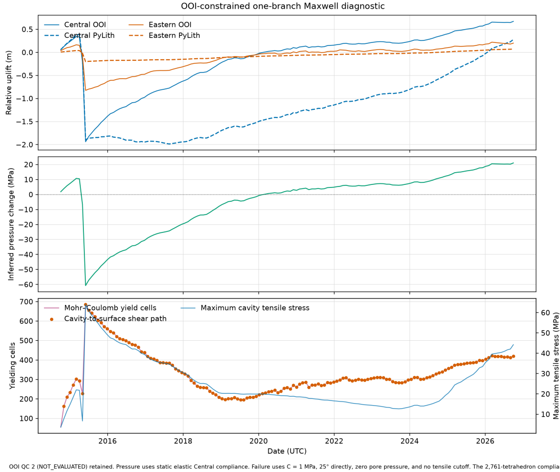
Figure 9: OOI-constrained one-branch Maxwell diagnostic. The panels compare OOI and modeled uplift, static-fit pressure, and stress-derived failure indicators. Generated by make ooi-maxwell-history-plot . Quality code 2 is retained; pressure uses static compliance; the mesh and failure assumptions remain provisional.
