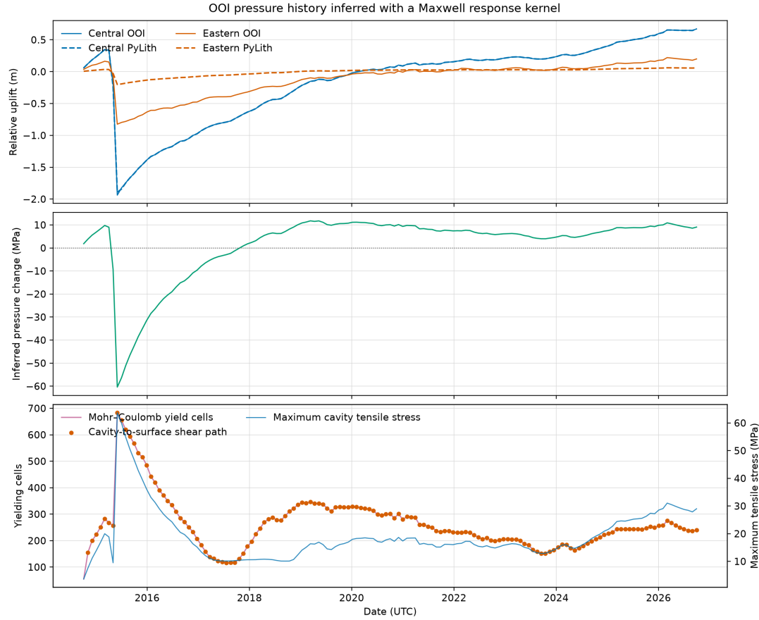
Figure 11: OOI Central pressure inversion with a one-branch Maxwell response kernel. Central is fitted and Eastern is held out; dashed curves show the direct PyLith history. The plot includes the inferred pressure and provisional failure diagnostics. Generated by make ooi-maxwell-pressure-inversion from independent OOI records. The smoothness prior, pressure scale, and nonconverged mesh remain provisional.
