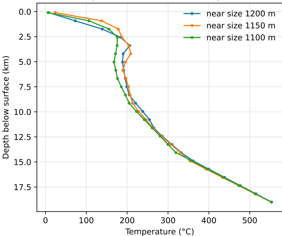
Temperature on the x = 5 km profile
