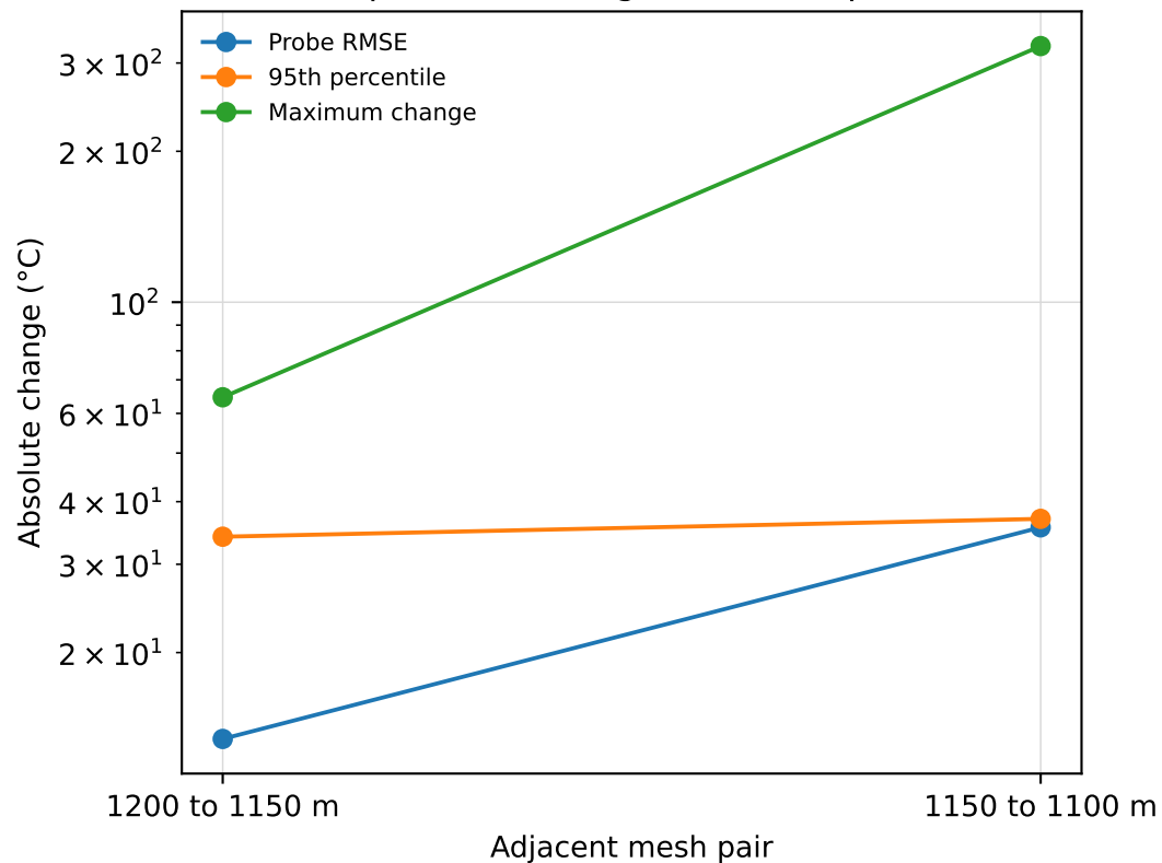
Temperature change at shared probes
