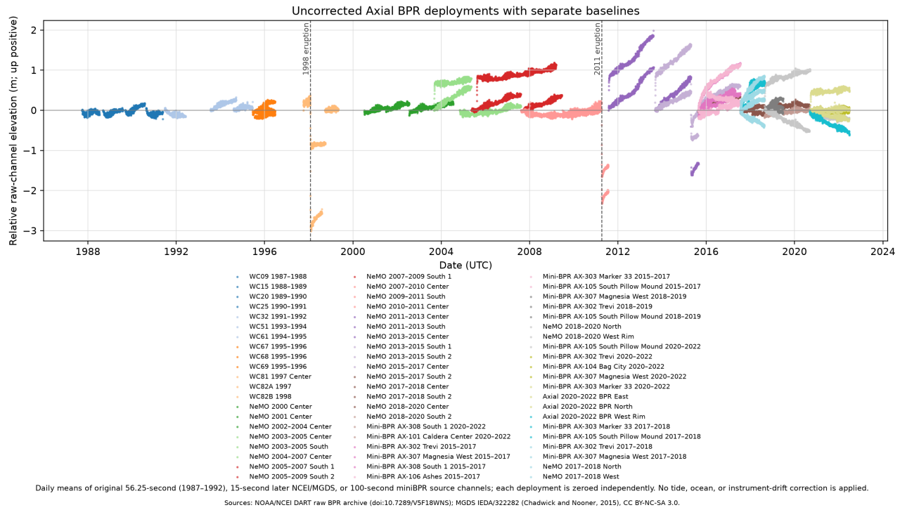
Figure 8: Separate-baseline daily means of original raw non-OOI BPR channels from 1987 through 2022. The plot shows intermittent deployment coverage; each segment is zeroed independently and remains uncorrected for tides, ocean variability, and instrument drift. Generated by make bpr-historical-check . Sources: NOAA/NCEI DART raw BPR archive (doi:10.7289/V5F18WNS) and MGDS IEDA/322282 (Chadwick and Nooner, 2015). MGDS-derived values are distributed under CC BY-NC-SA 3.0.
