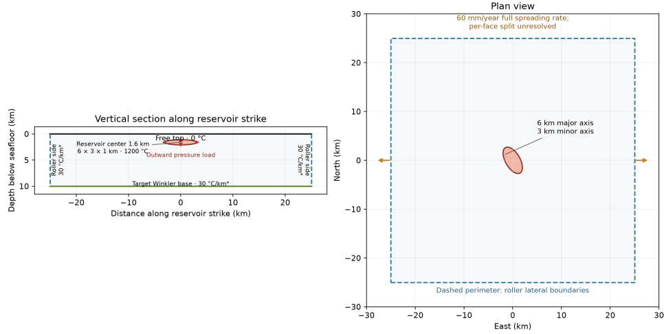
Figure 2: Schematic of the project-directed reservoir geometry and boundary conditions. The 50 by 50 km box extends from the seafloor to 10 km depth; reservoir dimensions and center depth follow the written specification. Roller sides, a Winkler base, a free top, and the 60 mm/year full spreading rate are labeled without assigning an unresolved per-face velocity. The 30 °C/km side and basal thermal conditions are project assumptions. Generated by make model-setup-schematic ; no published figure or geological data were used.
