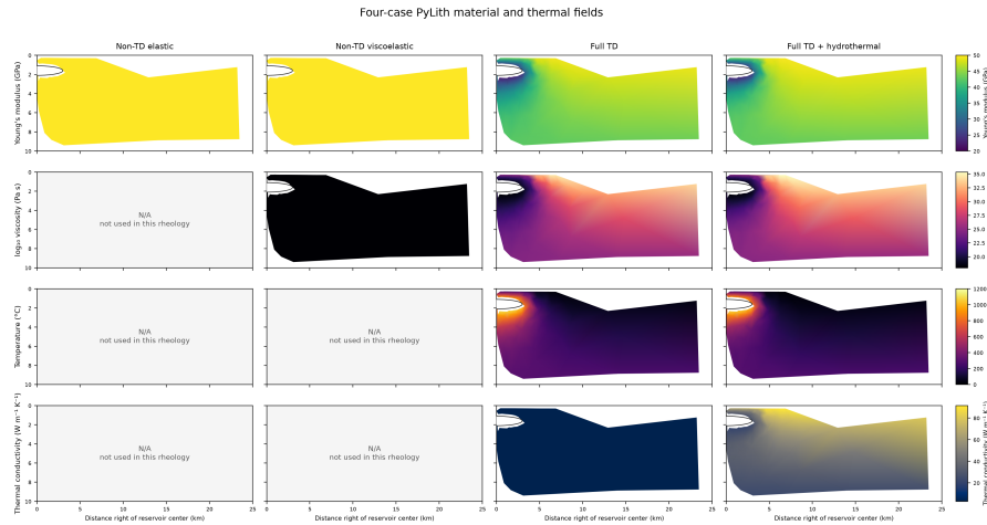
Figure 4: Project-generated four-case property matrix in the requested 4 by 4 layout. Rows show Young's modulus, log viscosity, temperature, and thermal conductivity; columns are non-temperature-dependent elastic, non-temperature-dependent viscoelastic, Full TD, and Full TD plus hydrothermal cases. The 50-to-20 GPa modulus mapping follows the project instruction, while Maxwell branch viscosities are synthetic. The maps cover the project-directed 50 by 50 km horizontal box and 0–10 km depth. These are PyLith property fields used by the bounded common 1 MPa, two-year diagnostic run, not Cabaniss output or a calibrated eruption prediction. The solve uses a fixed base pending a validated Axial Winkler foundation. Generated by make figure3-rheology-properties .
