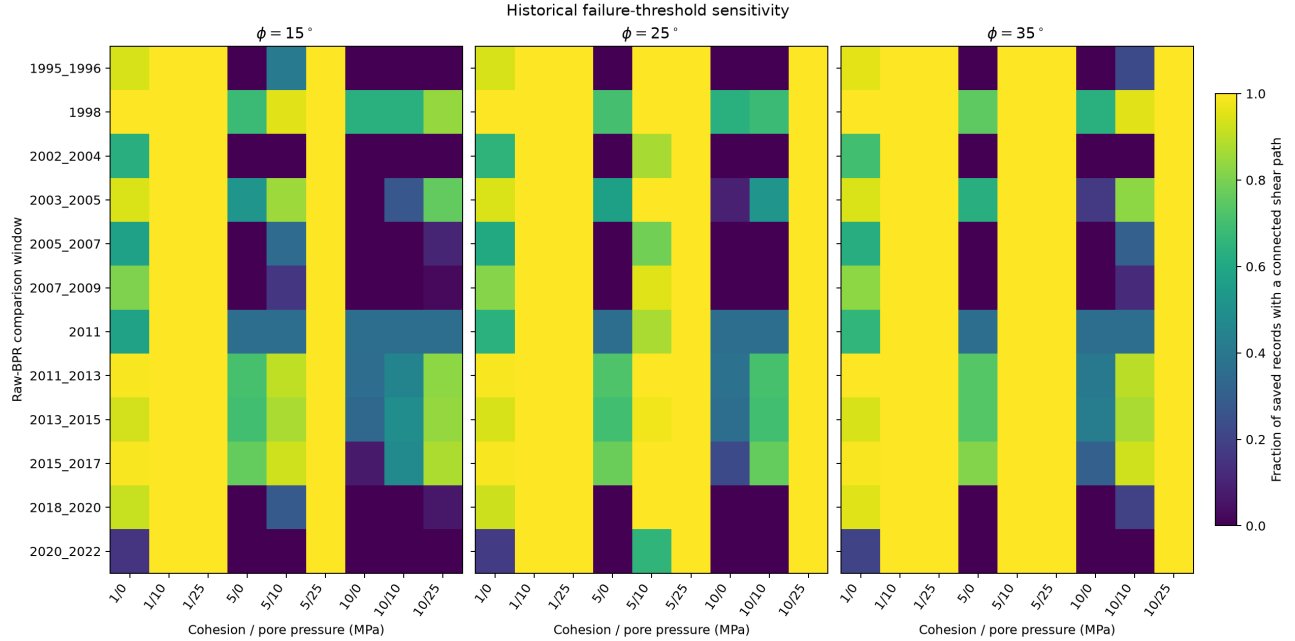
Figure 6: Fraction of saved records with a connected cavity-to-top shear path across a diagnostic grid of cohesion and pore pressure, shown for three direct friction angles. Zero-valued cells have no path in any saved record. The grid postprocesses independently generated raw-BPR-driven PyLith stress histories and does not assign tensile strength or calibrate rock properties. Generated by make historical-failure-threshold-sensitivity .
