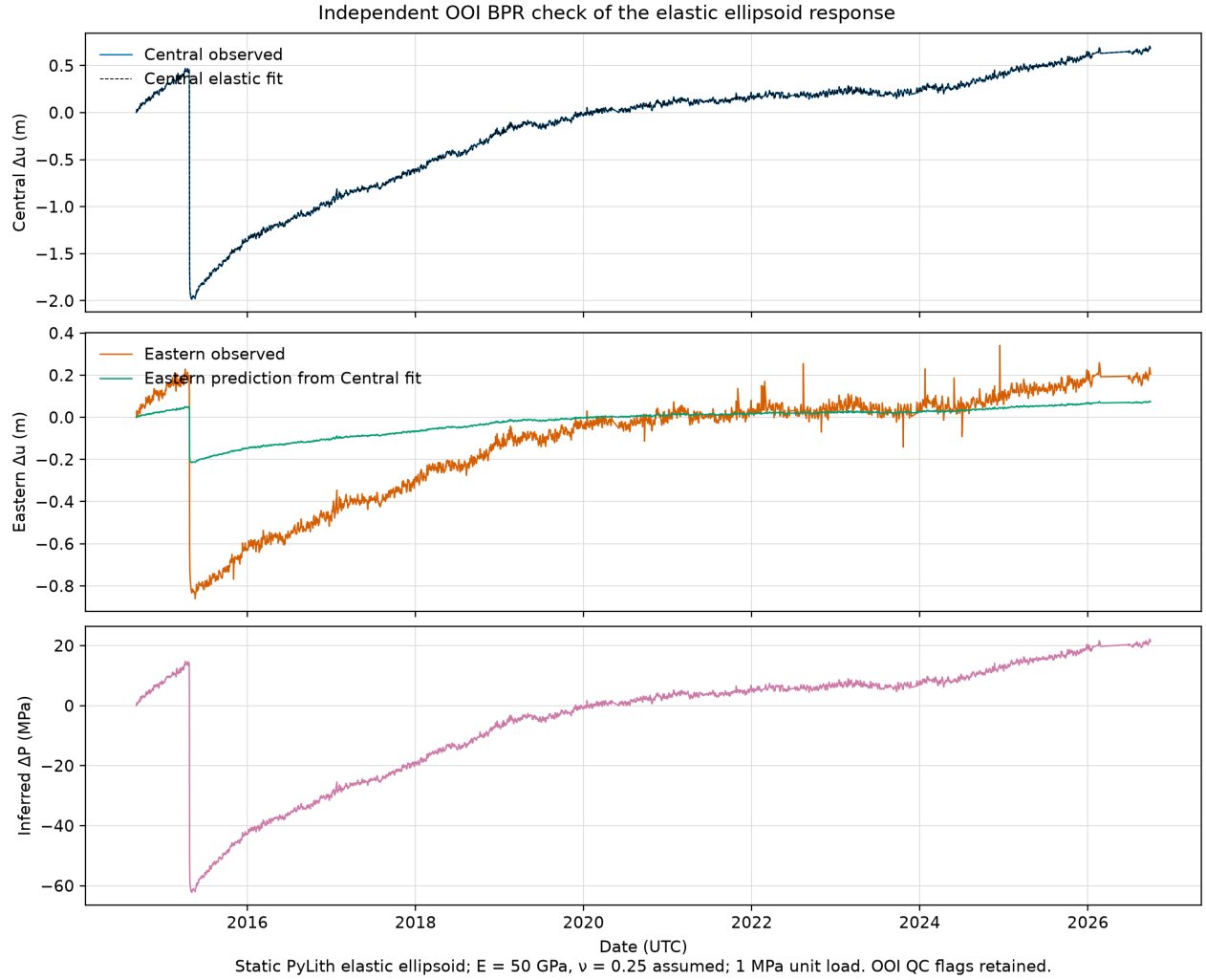
Figure 15: Static elastic ellipsoid fit to Central OOI uplift and Eastern holdout prediction. Generated by make ellipsoid-bpr-check . The amplitude mismatch and nonconverged compliance make the inferred pressure provisional.
