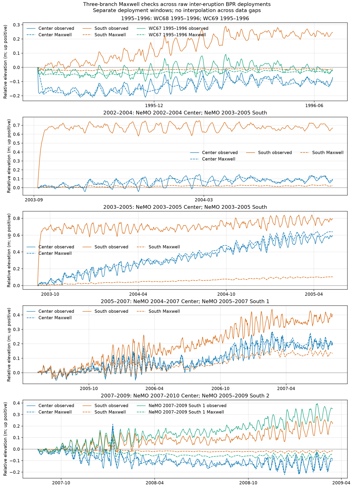
Figure 11: Three-branch Maxwell checks for raw Center/South deployment overlaps from 1995 through 2009. WC67 is held out in 1995–96 and NeMO South 1 in 2007–09. Each pair is independently zeroed; gaps are not interpolated. Generated by make reproduce .
