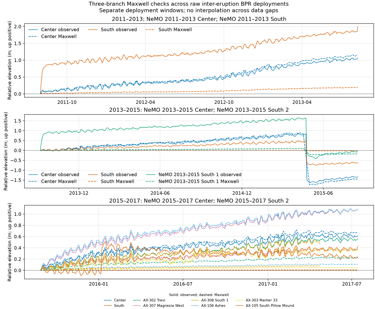
Figure 12: Three-branch Maxwell checks for raw Center/South deployment overlaps from 2011 through 2017. NeMO South 1 is held out for 2013–15. Each pair is independently zeroed; gaps are not interpolated. Center pressure uses static elastic compliance, and synthetic branch parameters and uncorrected records are diagnostic assumptions. The MGDS channels are original RawDep data from IEDA/322282, distributed under CC BY-NC-SA 3.0. Generated by make reproduce .
