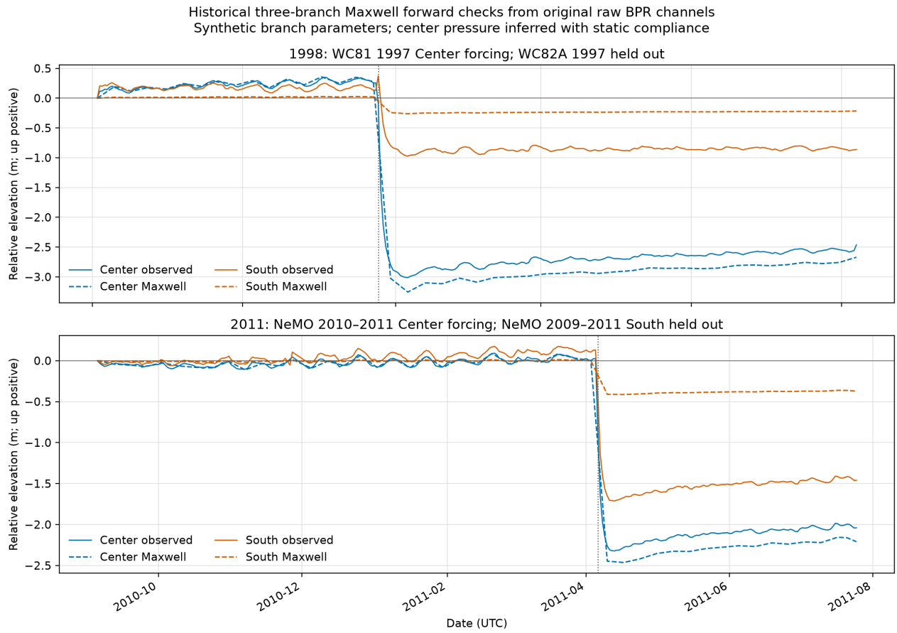
Figure 7: Three-branch generalized Maxwell forward checks against raw daily BPR observations for the 1998 and 2011 Center/South deployment pairs. Center pressure is inferred from static elastic compliance; South is held out. Synthetic branch properties, first-common-day zeroing, uncorrected raw records, and nonconverged compliance limit interpretation. Generated by make historical-generalized-maxwell-check .
