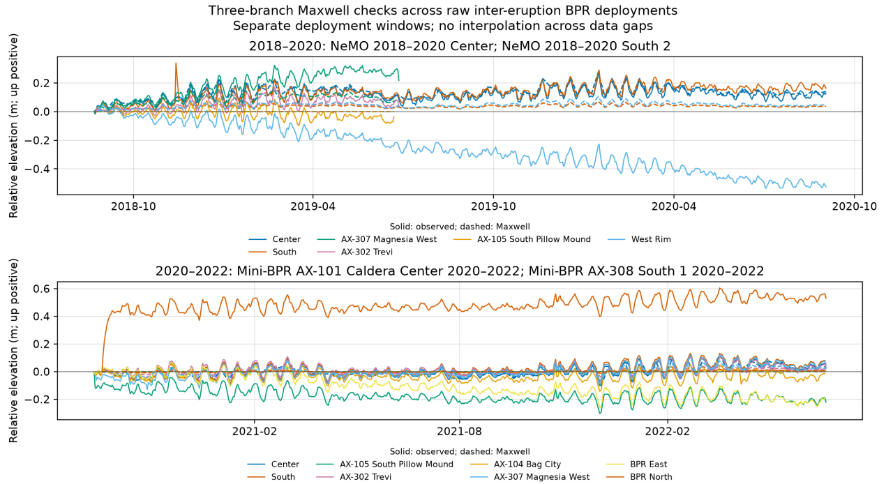
Figure 13: Three-branch Maxwell checks for original raw Center/South deployments from 2018 through 2022, with additional raw station holdouts in both panels. Solid lines are observations and dashed lines are Maxwell predictions. The upper panel includes 15-second moored-BPR Depth channels and 100-second miniBPR RawDepth channels; the lower panel includes 15-second moored-BPR Depth and 100-second miniBPR RawDepth(m) channels. Each station is independently zeroed, with no pressure-drift or tide correction. Documented location and quality issues are excluded as described in Table 4. Generated by make historical-post-2017-bpr-check .
