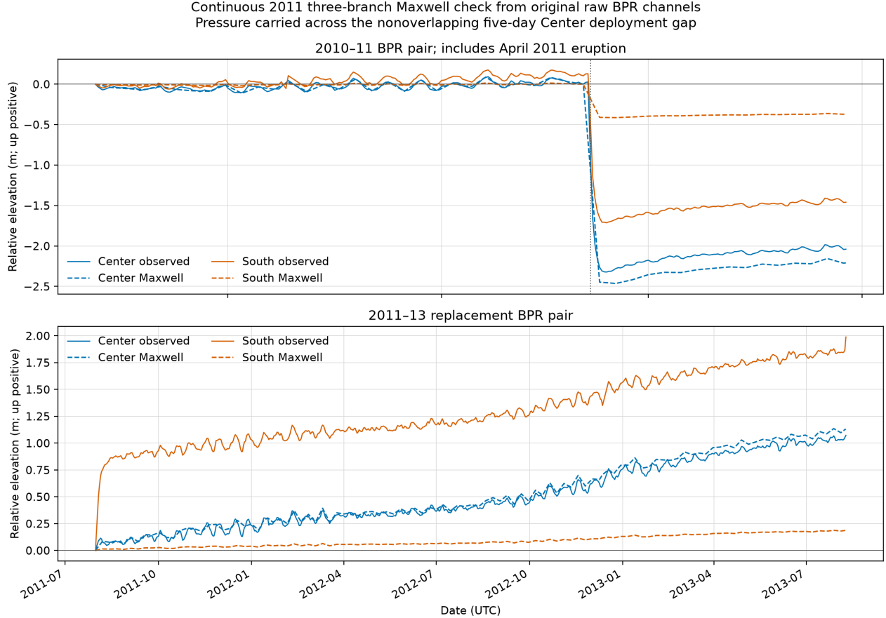
Figure 8: Continuous 2011 three-branch Maxwell check from original raw MGDS BPR channels. Each panel shows Center-forced predictions and its paired South holdout, independently baselined by deployment. The Center pressure series are joined across a five-day gap by holding the final pressure constant. The eruption date is marked in the upper panel. Synthetic branch parameters, raw instrument effects, and nonconverged compliance limit interpretation. Source channels: MGDS IEDA/322282 (Chadwick et al., 2023), CC BY-NC-SA 3.0. Generated by make historical-generalized-maxwell-2011-continuous-check .
