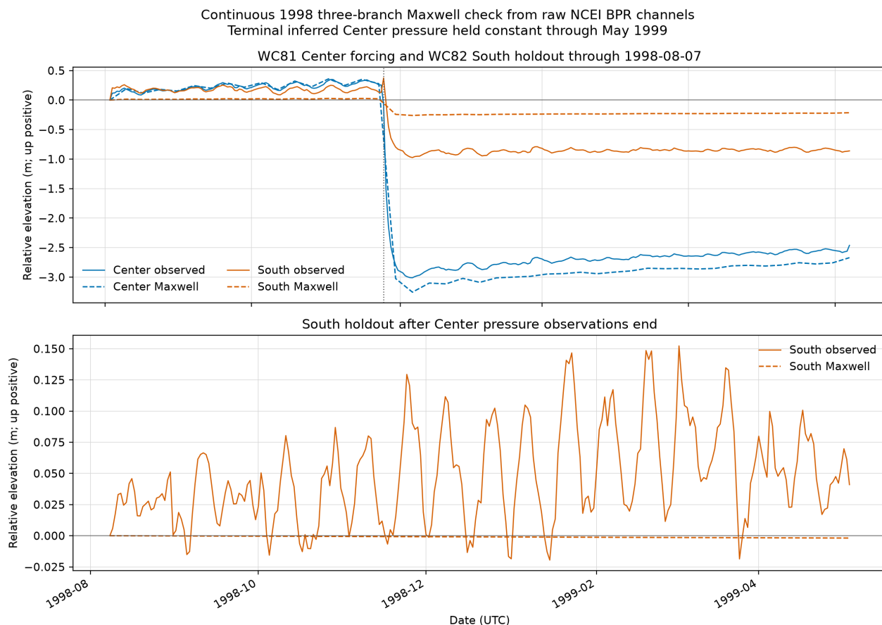
Figure 9: Continuous 1998 three-branch Maxwell check using only original NCEI WC81 Center and WC82 South absolute-pressure channels. The upper panel compares Center forcing and the event South holdout through 7 August 1998; the lower panel checks the South station through 4 May 1999 after Center pressure observations end. The two WC82 South files are aligned from their eight-day raw overlap. Terminal inferred Center pressure is held constant for 270 days. Synthetic branch parameters, raw ocean variability, and nonconverged compliance limit interpretation. Source: NCEI DART raw BPR archive, doi:10.7289/V5F18WNS. Generated by make historical-generalized-maxwell-1998-continuous-check .
