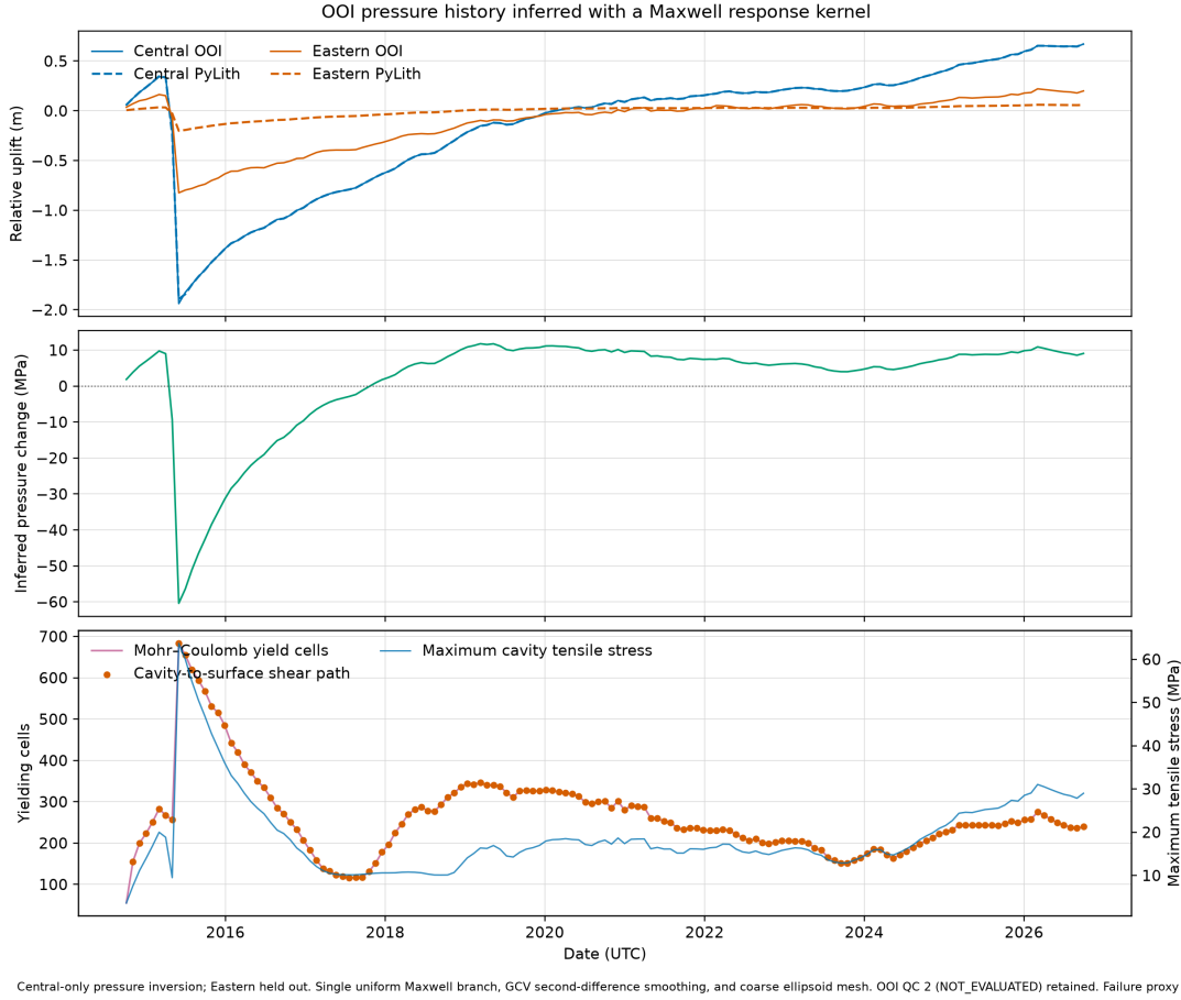
Figure 17: OOI Central pressure inversion with a one-branch Maxwell response kernel. Central is fitted and Eastern is held out; dashed curves show the direct PyLith history. The plot includes the inferred pressure and provisional failure diagnostics. Generated by make ooi-maxwell-pressure-inversion from independent OOI records. The smoothness prior, pressure scale, and nonconverged mesh remain provisional.
