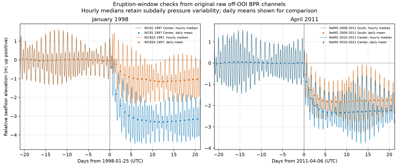
Figure 19: Hourly medians and daily means from original raw off-OOI BPR channels around the 1998 and 2011 events. Each station has its own baseline from days -7 through -1 ; hours require 75 percent sample coverage. No tidal, oceanographic, filter, or drift correction is applied. Vertical markers show the event date at day-level resolution and do not estimate an eruption time. Generated by make_historical-bpr-subdaily-event-check from raw NOAA/NCEI dbar and MGDS RawDep/Depth channels. Sources: NOAA/NCEI (doi:10.7289/V5F18WNS) and original MGDS IEDA/322282 channels (William Chadwick, Scott Nooner, and MGDS; CC BY-NC-SA 3.0).
