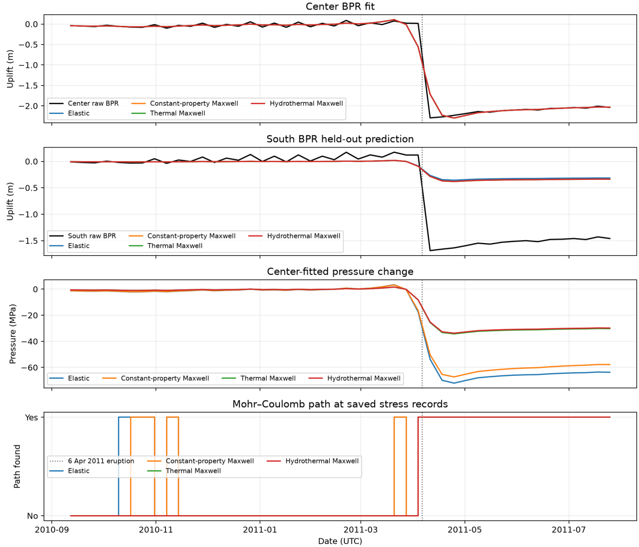
Figure 16: Four pressure calibrations against original raw NeMO Center BPR data, with NeMO South held out and provisional connected-path states shown at saved stress records. Dotted vertical lines mark the observed 6 April 2011 eruption. Each pressure history is fitted independently; the Center input includes the eruption deflation and subsequent data. Synthetic branch parameters, the nonconverged mesh, and unresolved failure assumptions make this a retrospective diagnostic. Generated by make historical-four-case-bpr-calibration . Sources are original MGDS IEDA/322282 RawDep/Depth channels (William Chadwick, Scott Nooner, and MGDS; CC BY-NC-SA 3.0).
