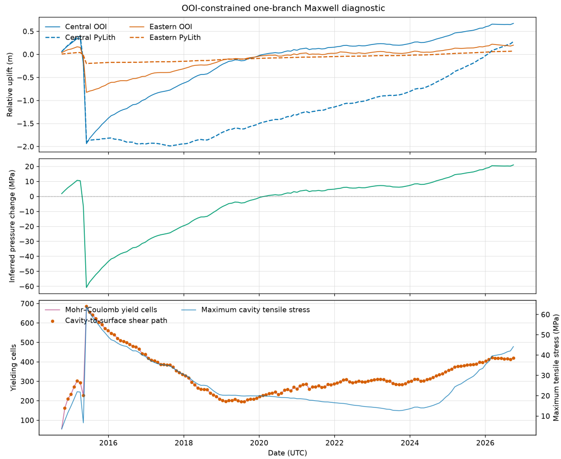
Figure 6: OOI-constrained one-branch Maxwell diagnostic. The panels compare OOI and modeled uplift, static-fit pressure, and stress-derived failure indicators. Generated by make ooi-maxwell-history-plot . Quality code 2 is retained; pressure uses static compliance; the mesh and failure assumptions remain provisional.
