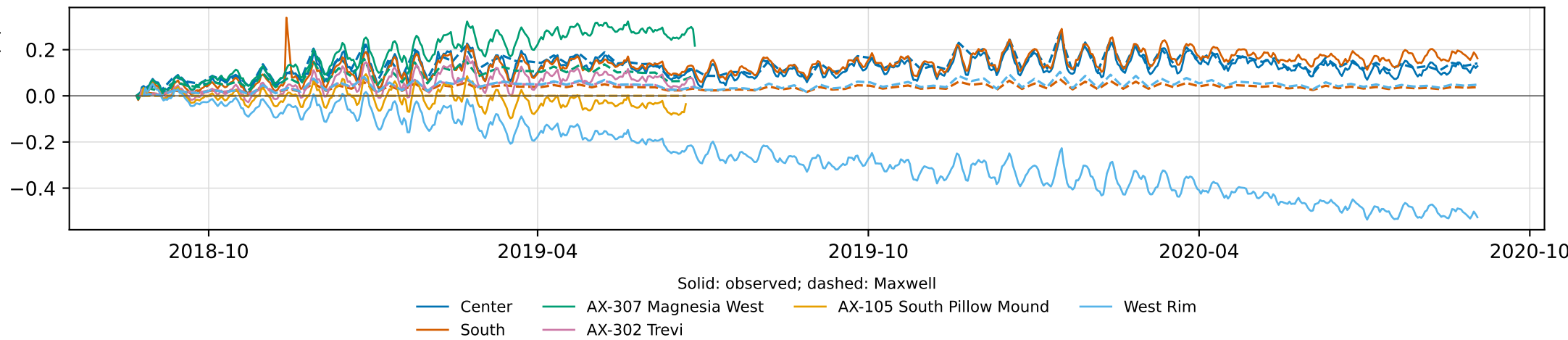
Three-branch Maxwell checks across raw inter-eruption BPR deployments Separate deployment windows; no interpolation across data gaps 2018-2020: NeMO 2018-2020 Center; NeMO 2018-2020 South 2
