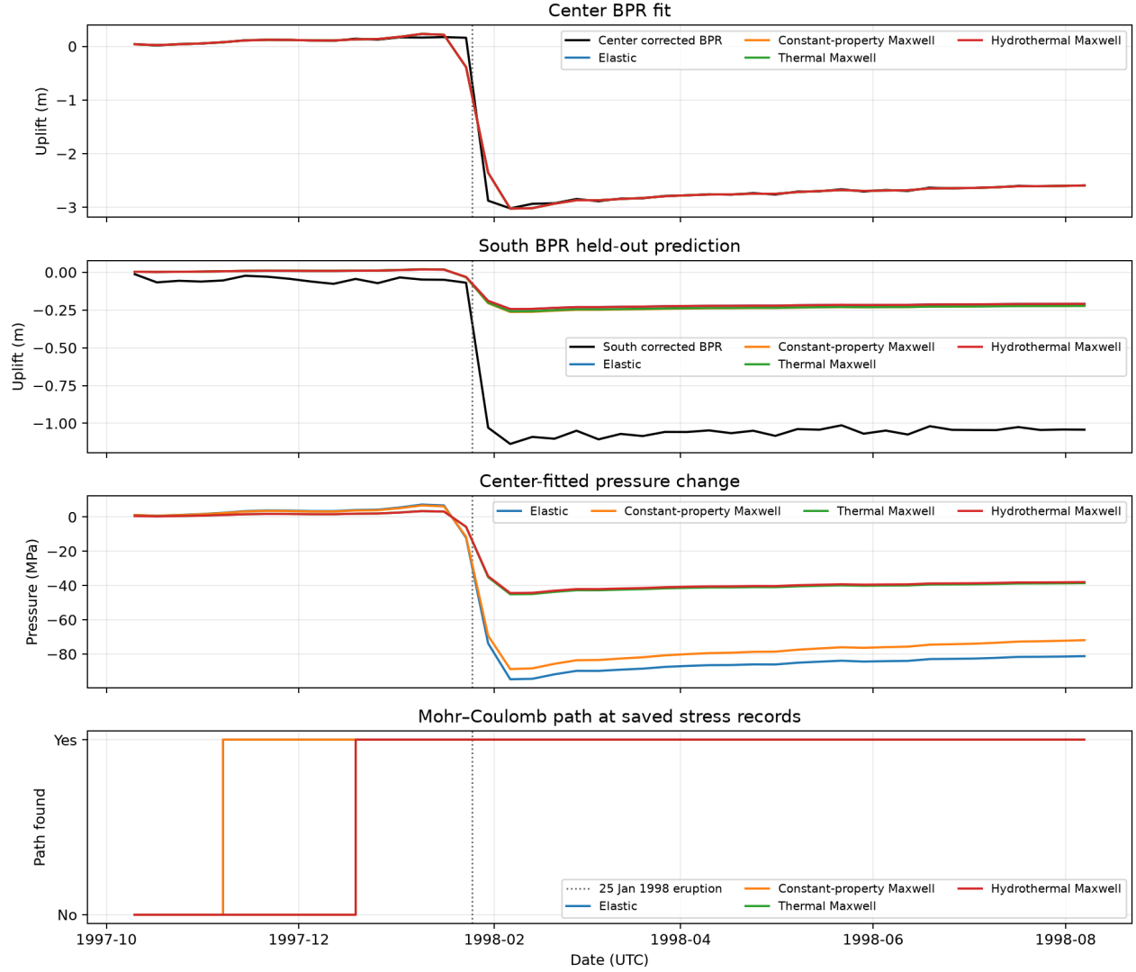
Figure 22: Four rheology fits to the MGDS Fox 1997–98 tide-corrected Center channel Spot1DetidedDepth , with the tide-corrected South channel held out. Neither channel has an MPR drift estimate. The panels show Center fit, South prediction, inferred Center pressure, and saved-record failure paths. The Center fit includes eruption deflation and later observations. Sources: MGDS IEDA/322344, Fox (2016), CC BY-NC-SA 3.0.
