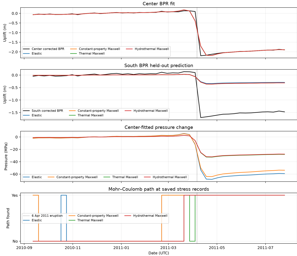
Figure 23: Four rheology fits to the MGDS NeMO 2010–11 Center DriftCorrSpot1Dep channel, corrected for predicted tide and MPR drift, with the tide-corrected 2009–11 South Spot1DetidedDepth channel held out. Non-tidal ocean variability remains. The Center fit includes eruption deflation and subsequent observations. Sources: MGDS IEDA/322282, Chadwick et al. (2023), CC BY-NC-SA 3.0.
