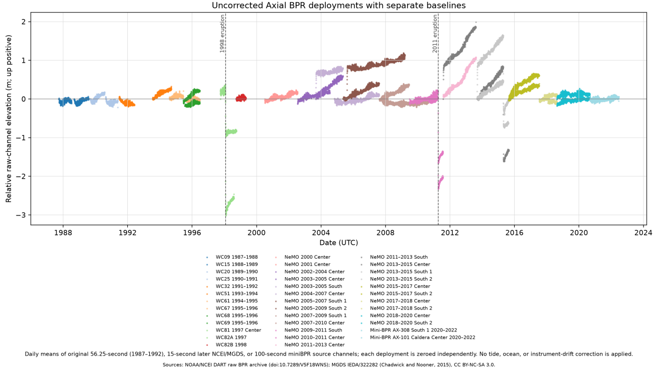
Figure 4: Separate-baseline daily means of original raw non-OOI BPR channels from 1987 through 2022. The plot shows intermittent deployment coverage; each segment is zeroed independently and remains uncorrected for tides, ocean variability, and instrument drift. Generated by make bpr-historical-check . Sources: NOAA/NCEI DART raw BPR archive (doi:10.7289/V5F18WNS) and MGDS IEDA/322282 (Chadwick and Nooner, 2015). MGDS-derived values are distributed under CC BY-NC-SA 3.0.
