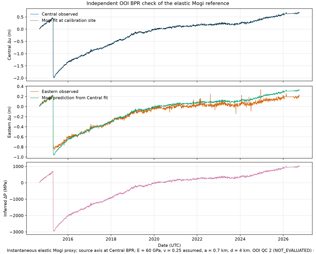
Figure 11: OOI observations and elastic Mogi point-source response. Generated by make bpr-mogi-check from independent OOI records; Central is fit by construction and Eastern is held out. The inferred pressure scale is physically unsuitable for the later reservoir model.
