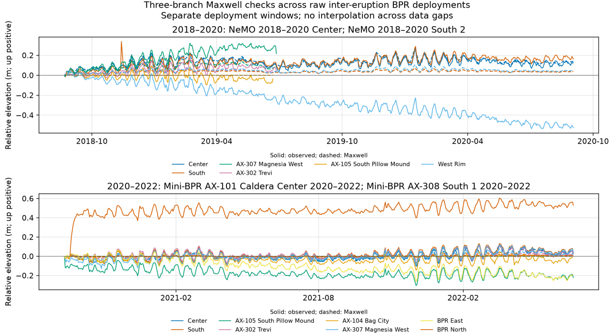
Figure 10: Three-branch Maxwell checks for original raw Center/South deployments from 2018 through 2022, with additional raw station holdouts in both panels. Solid lines are observations and dashed lines are Maxwell predictions. The upper panel includes 15-second moored-BPR Depth channels and 100-second miniBPR RawDep channels; the lower panel includes 15-second moored-BPR Depth and 100-second miniBPR RawDepth(m) channels. Each station is independently zeroed, with no pressure-drift or tide correction. Documented location and quality issues are excluded as described in Table 4. Generated by make_historical-post-2017-bpr-check .
