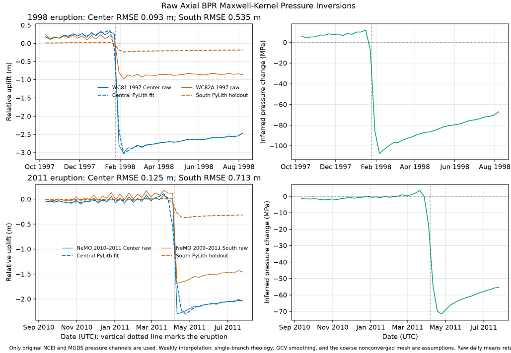
Figure 15: Maxwell-kernel pressure inversions of original raw BPR data across the 1998 and 2011 eruptions. Solid curves are uncorrected daily observations; dashed curves show the Central fit and held-out South prediction. Vertical dotted lines mark the eruption dates. Generated by make_historical-bpr-maxwell-pressure-inversion . Sources are NOAA/NCEI DART raw channels (doi:10.7289/V5F18WNS) and original MGDS IEDA/322282 Depth/RawDep channels (William Chadwick, Scott Nooner, and MGDS; CC BY-NC-SA 3.0).
