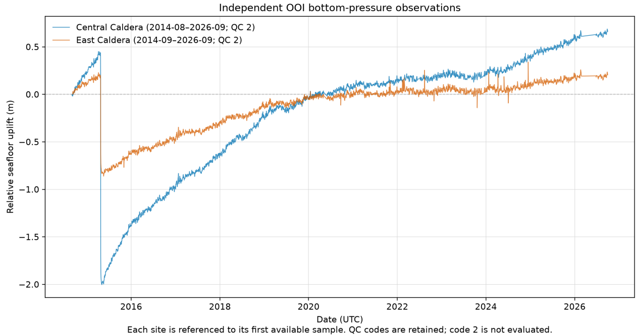
Figure 2: Daily OOI relative uplift at Central and Eastern Caldera from each site’s first available record. Generated by make bpr-observation-plot ; aggregate quality code 2 (NOT EVALUATED) is retained. The data show the observed interval available for independent model checking.
