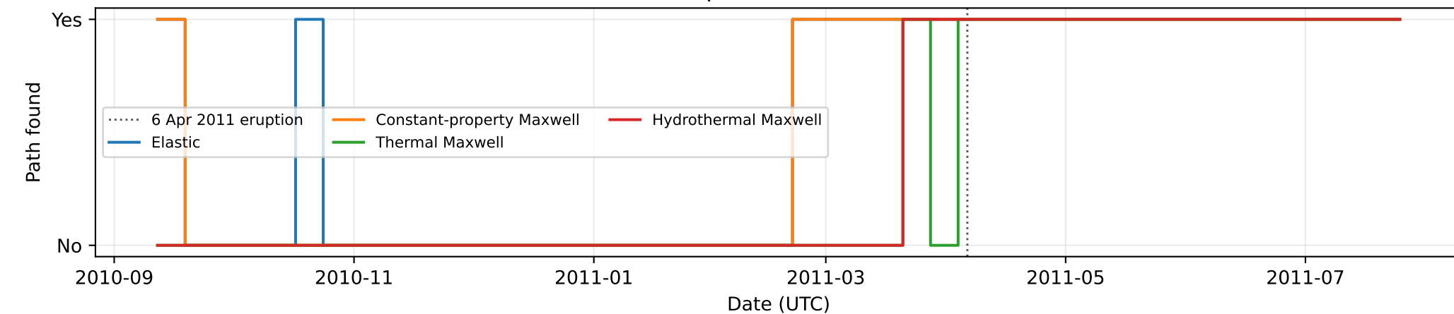
Mohr-Coulomb path at saved stress records
