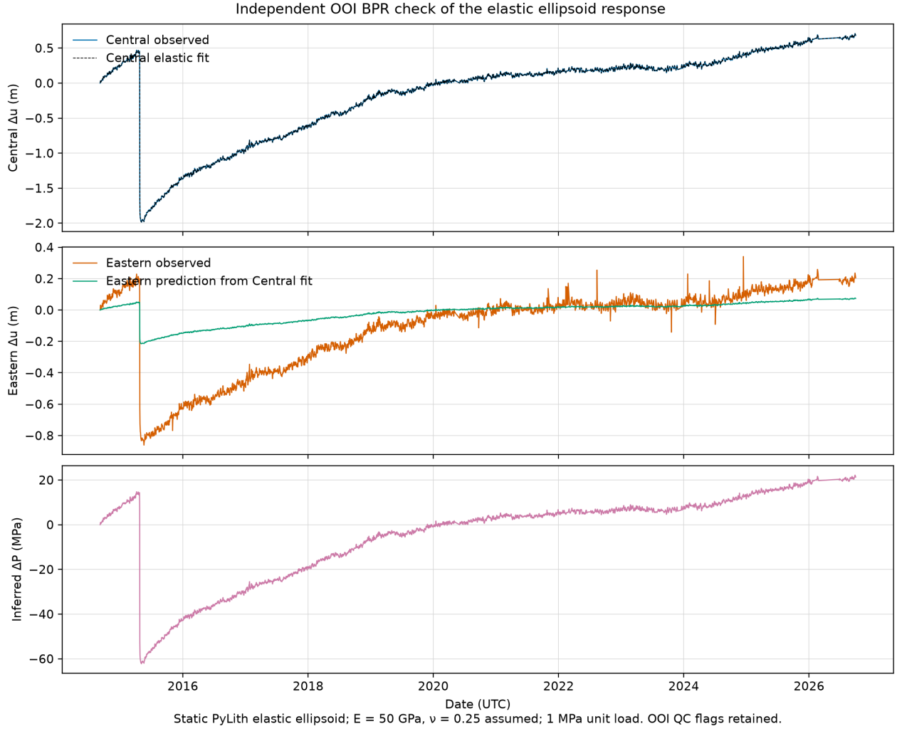
Figure 7: Static elastic ellipsoid fit to Central OOI uplift and Eastern holdout prediction. Generated by make ellipsoid-bpr-check . The amplitude mismatch and nonconverged compliance make the inferred pressure provisional.
