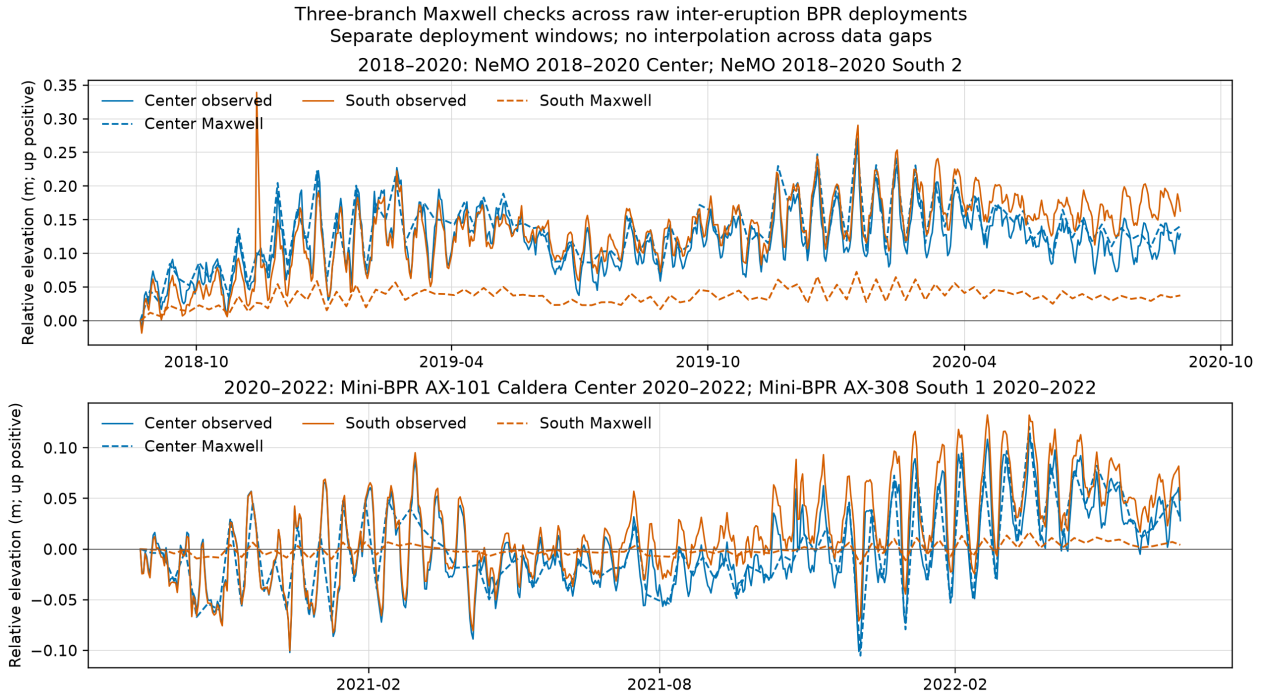
Figure 10: Three-branch Maxwell checks for original raw Center/South deployments from 2018 through 2022. The upper panel uses the 15-second moored-BPR RawDep channels; the lower panel uses the 100-second miniBPR RawDepth(m) channels. Each pair is independently zeroed, with no pressure-drift or tide correction. Generated by make_historical-post-2017-bpr-check .
