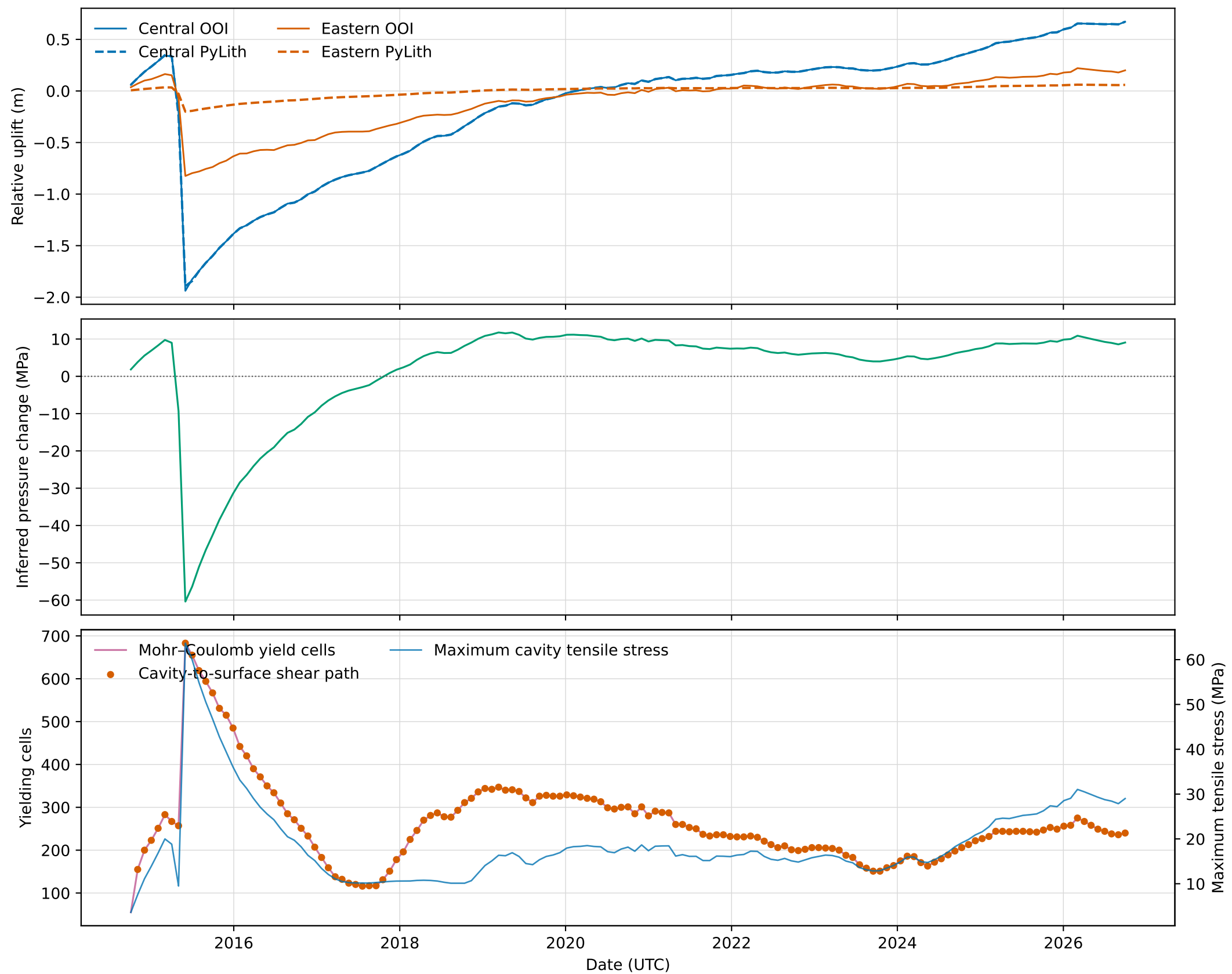
OOI pressure history inferred with a Maxwell response kernel
