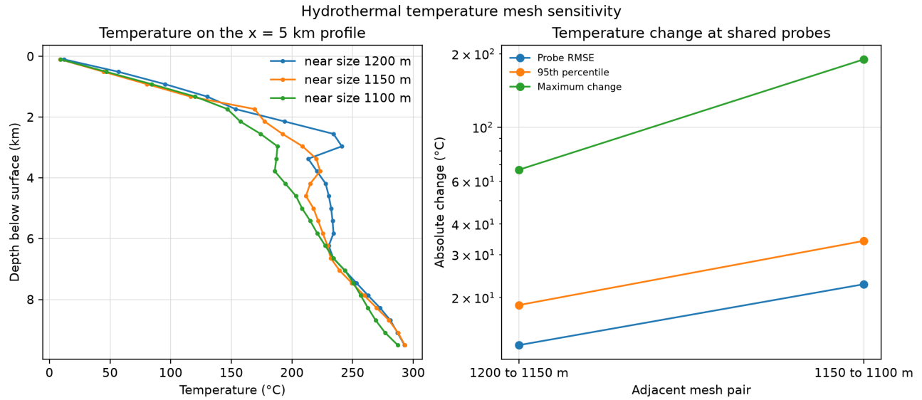
Figure 6: Hydrothermal temperature sensitivity across three bounded tetrahedral meshes. The left panel shows interpolated temperatures along a common vertical profile. The right panel shows RMSE, 95th-percentile, and maximum absolute changes across 105 common host-rock probes for adjacent meshes. Meshes are independently generated and non-nested; the probe changes diagnose spatial sensitivity but do not establish convergence. Generated by make thermal-mesh-sensitivity .
