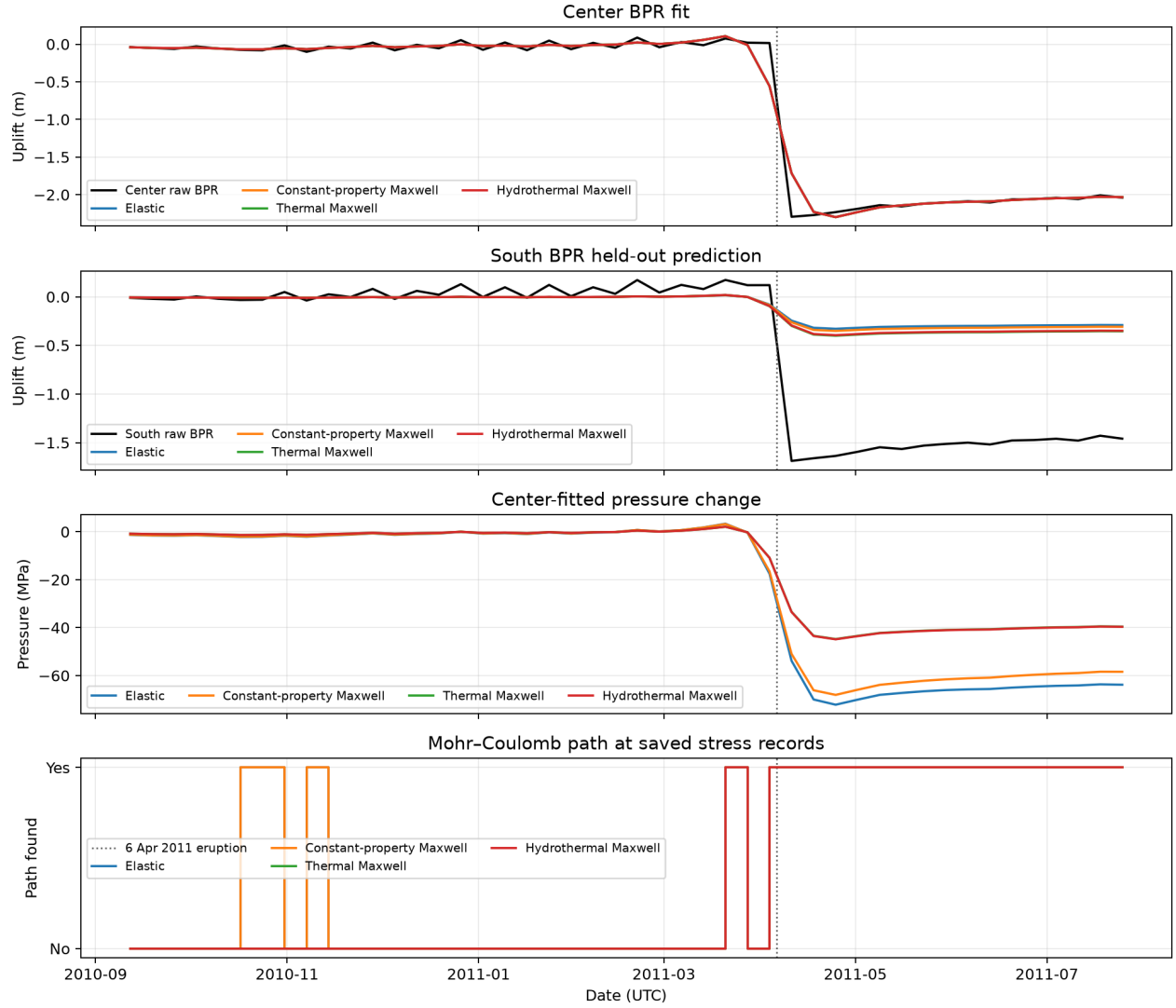
Figure 24: Four pressure calibrations against original raw NeMO Center BPR data, with NeMO South held out and provisional connected-path states shown at saved stress records. Dotted vertical lines mark the observed 6 April 2011 eruption. Each pressure history is fitted independently; the Center input includes the eruption deflation and subsequent data. Synthetic branch parameters, the nonconverged mesh, and unresolved failure assumptions make this a retrospective diagnostic. Generated by make historical-four-case-bpr-calibration . Sources are original MGDS IEDA/322282 RawDep/Depth channels (William Chadwick, Scott Nooner, and MGDS; CC BY-NC-SA 3.0).
