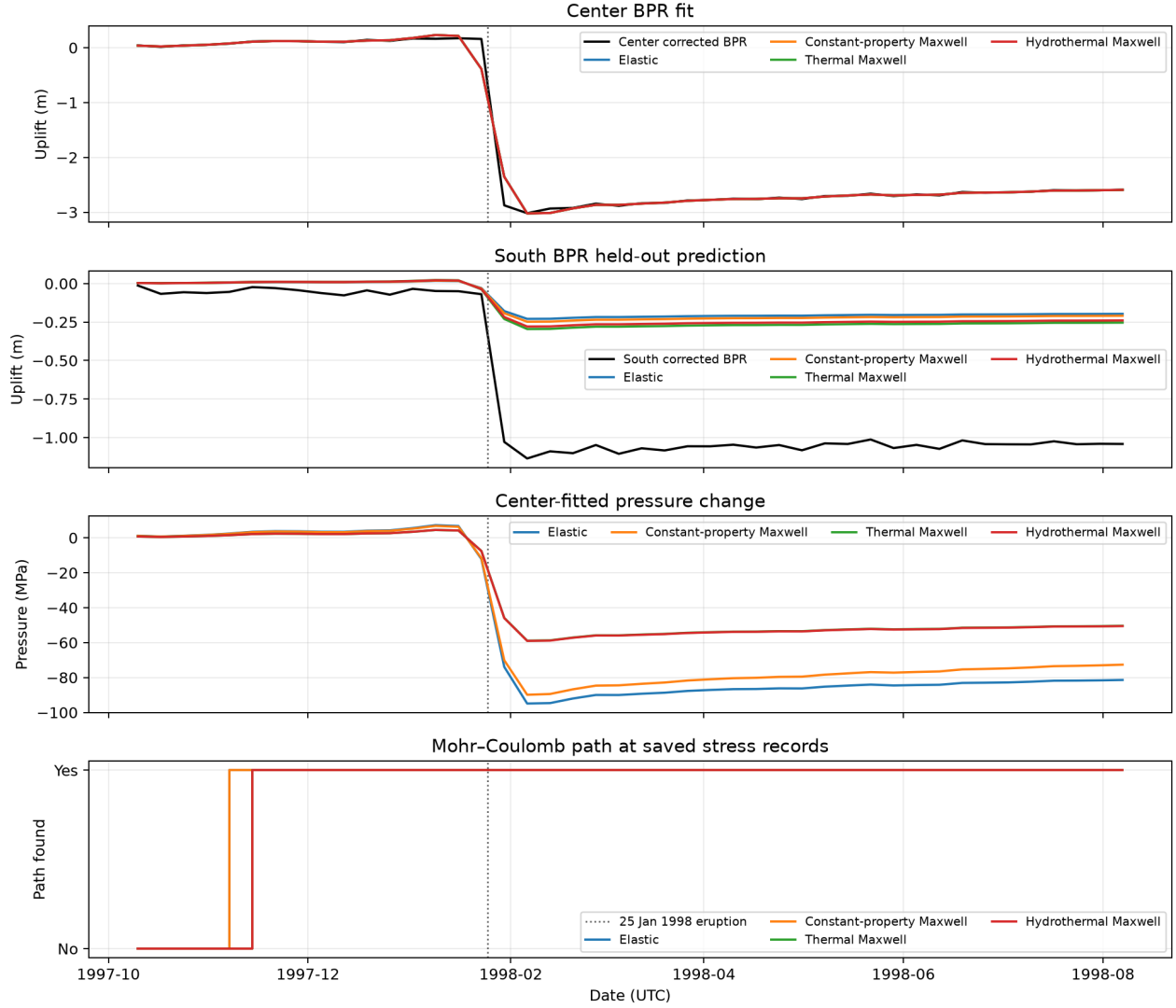
Figure 25: Four rheology fits to the MGDS Fox 1997–98 tide-corrected Center channel Spot1DetidedDepth , with the tide-corrected South channel held out. Neither channel has an MPR drift estimate. The panels show Center fit, South prediction, inferred Center pressure, and saved-record failure paths. The Center fit includes eruption deflation and later observations. Sources: MGDS IEDA/322344, Fox (2016), CC BY-NC-SA 3.0.
