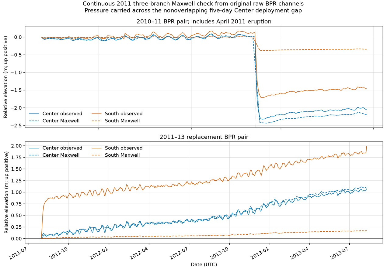
Figure 11: Continuous 2011 three-branch Maxwell check from original raw MGDS BPR channels. Each panel shows Center-forced predictions and its paired South holdout, independently baselined by deployment. The Center pressure series are joined across a five-day gap by holding the final pressure constant. The eruption date is marked in the upper panel. Synthetic branch parameters, raw instrument effects, and nonconverged compliance limit interpretation. Source channels: MGDS IEDA/322282 (Chadwick et al., 2023), CC BY-NC-SA 3.0. Generated by make historical-generalized-maxwell-2011-continuous-check .
