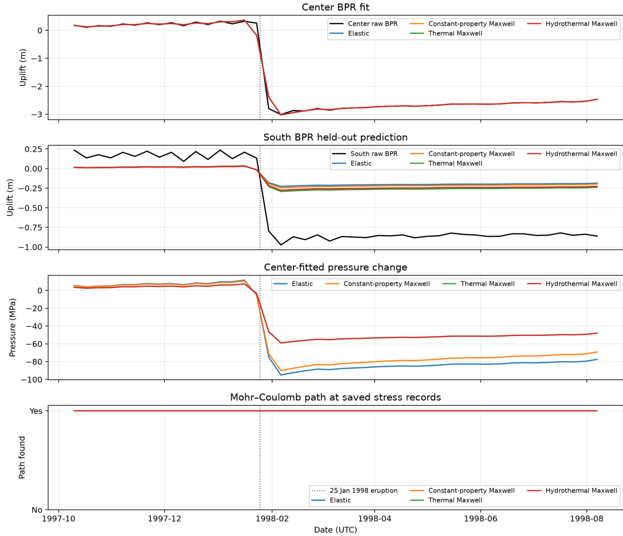
Figure 23: Four pressure calibrations against original raw NCEI WC81 Center data, with WC82A South held out and provisional connected-path states shown at saved stress records. The dotted line marks the observed 25 January 1998 eruption. Each pressure history is fitted independently, and Center includes the eruption deflation and later records. Synthetic branch parameters, the nonconverged mesh, and unresolved failure assumptions make this a retrospective diagnostic. No MGDS Fox duplicate or Cabaniss-associated data products were used. Generated by make historical-four-case-bpr-calibration .
