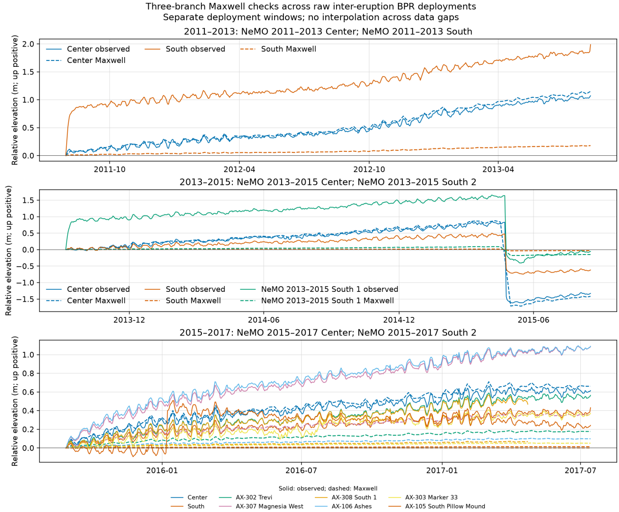
Figure 15: Three-branch Maxwell checks for raw Center/South deployment overlaps from 2011 through 2017. NeMO South 1 is held out for 2013–15. Each pair is independently zeroed; gaps are not interpolated. Center pressure uses static elastic compliance, and synthetic branch parameters and uncorrected records are diagnostic assumptions. The MGDS channels are original RawDep data from IEDA/322282, distributed under CC BY-NC-SA 3.0. Generated by make reproduce .
