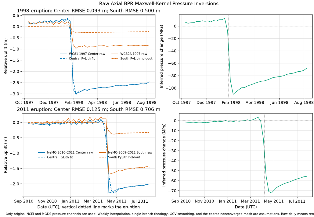
Figure 21: Maxwell-kernel pressure inversions of original raw BPR data across the 1998 and 2011 eruptions. Solid curves are uncorrected daily observations; dashed curves show the Central fit and held-out South prediction. Vertical dotted lines mark the eruption dates. Generated by make_historical-bpr-maxwell-pressure-inversion . Sources are NOAA/NCEI DART raw channels (doi:10.7289/V5F18WNS) and original MGDS IEDA/322282 Depth/RawDep channels (William Chadwick, Scott Nooner, and MGDS; CC BY-NC-SA 3.0).
