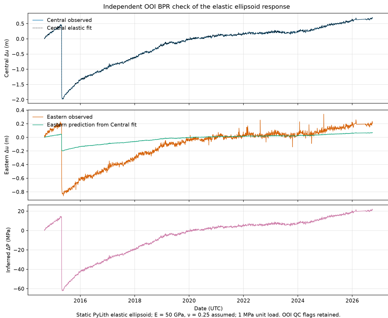
Figure 18: Static elastic ellipsoid fit to Central OOI uplift and Eastern holdout prediction. Generated by make ellipsoid-bpr-check . The amplitude mismatch and nonconverged compliance make the inferred pressure provisional.
