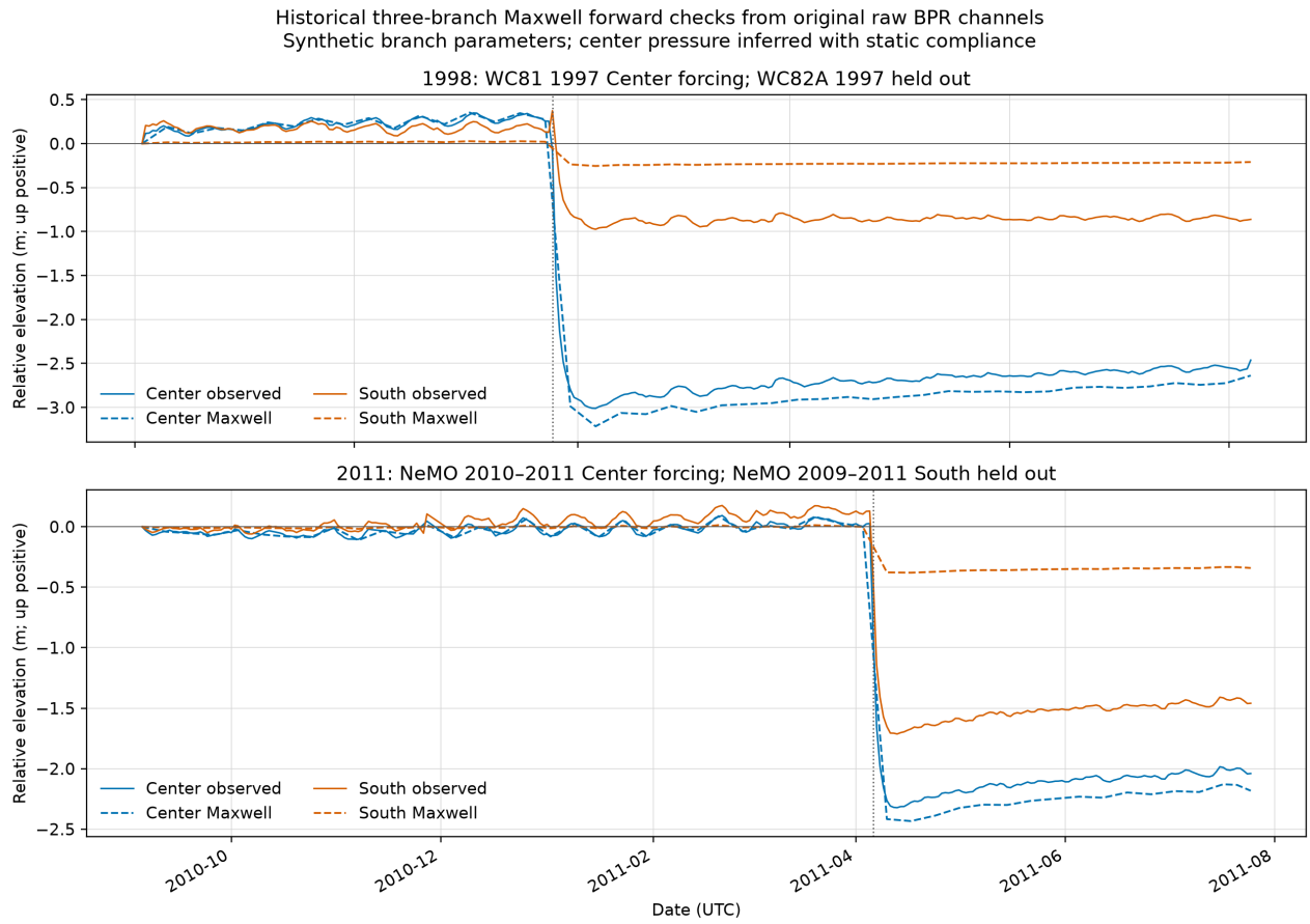
Figure 10: Three-branch generalized Maxwell forward checks against raw daily BPR observations for the 1998 and 2011 Center/South deployment pairs. Center pressure is inferred from static elastic compliance; South is held out. Synthetic branch properties, first-common-day zeroing, uncorrected raw records, and nonconverged compliance limit interpretation. Generated by make historical-generalized-maxwell-check .
