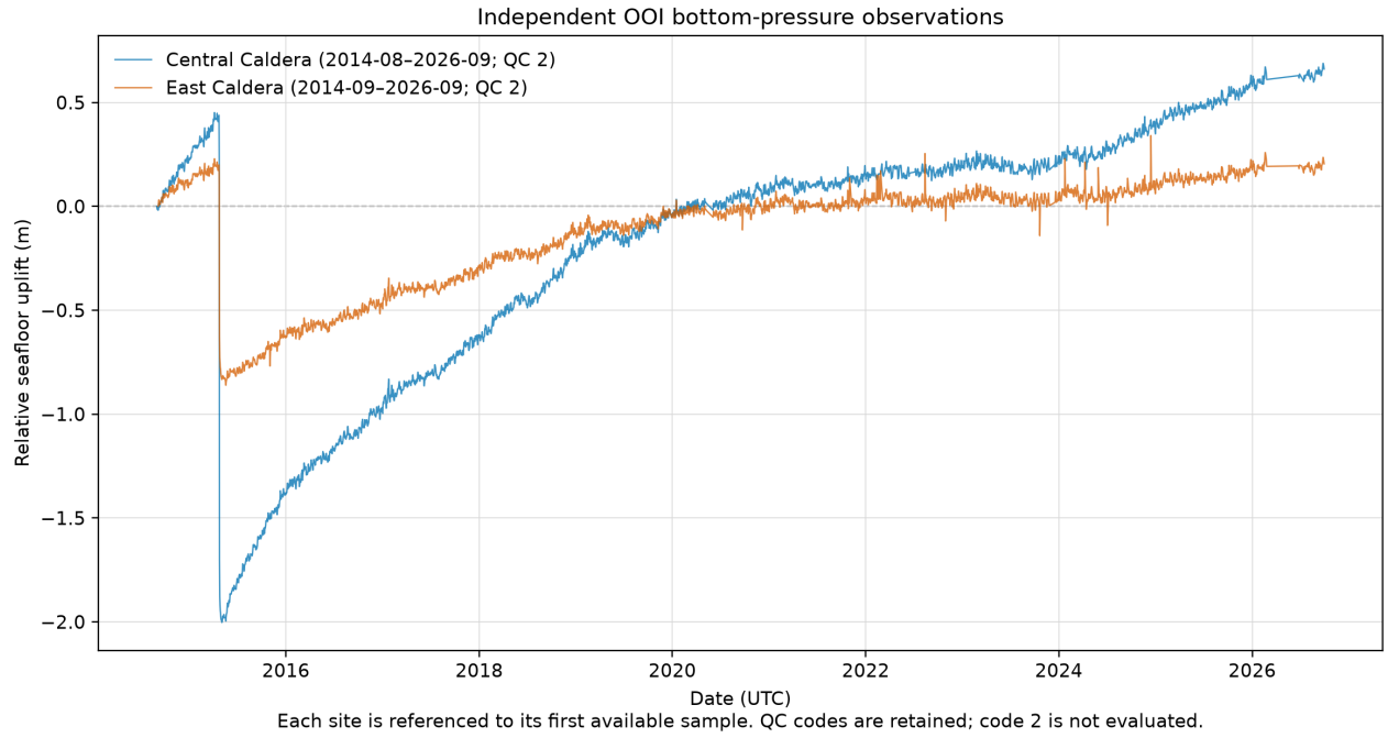
Figure 7: Daily OOI relative uplift at Central and Eastern Caldera from each site's first available record. Generated by make bpr-observation-plot ; aggregate quality code 2 (NOT EVALUATED) is retained. The data show the observed interval available for independent model checking.
