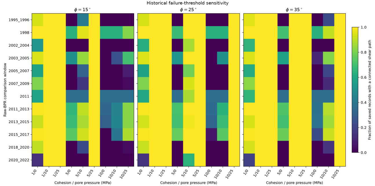
Figure 9: Fraction of saved records with a connected cavity-to-top shear path across a diagnostic grid of cohesion and pore pressure, shown for three direct friction angles. Zero-valued cells have no path in any saved record. The grid postprocesses independently generated raw-BPR-driven PyLith stress histories and does not assign tensile strength or calibrate rock properties. Generated by make historical-failure-threshold-sensitivity .
