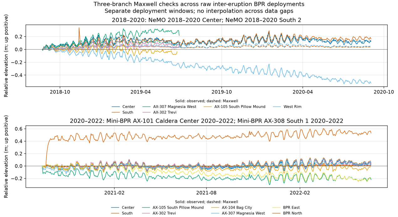
Figure 16: Three-branch Maxwell checks for original raw Center/South deployments from 2018 through 2022, with additional raw station holdouts in both panels. Solid lines are observations and dashed lines are Maxwell predictions. The upper panel includes 15-second moored-BPR Depth channels and 100-second miniBPR RawDep channels; the lower panel includes 15-second moored-BPR Depth and 100-second miniBPR RawDepth(m) channels. Each station is independently zeroed, with no pressure-drift or tide correction. Documented location and quality issues are excluded as described in Table 4. Generated by make historical-post-2017-bpr-check .
