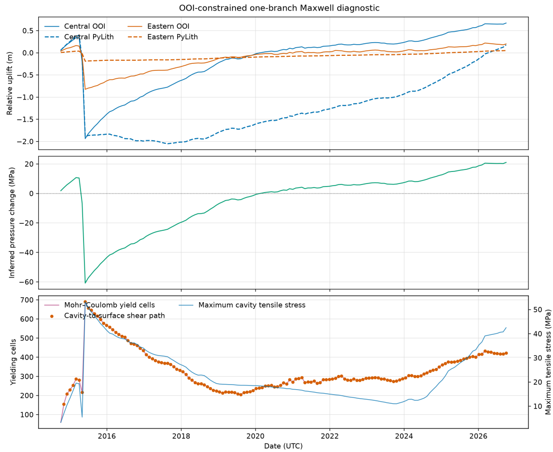
Figure 19: OOI-constrained one-branch Maxwell diagnostic. The panels compare OOI and modeled uplift, static-fit pressure, and stress-derived failure indicators. Generated by make ooi-maxwell-history-plot . Quality code 2 is retained; pressure uses static compliance; the mesh and failure assumptions remain provisional.
