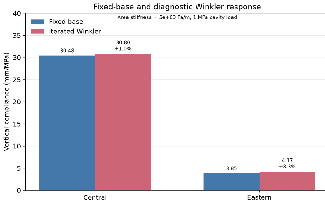
Figure 3: Vertical compliance under a 1 MPa cavity load for the fixed-base reference and the separate outer-iteration Winkler diagnostic. Bars show Central and Eastern surface displacement per unit pressure; labels above the Winkler bars give the percent change from the fixed-base values. The check uses one coarse shared mesh and an illustrative spring coefficient, not an Axial estimate. It does not resolve the density contrast or basal prestress. Generated by make winkler-foundation-check .
