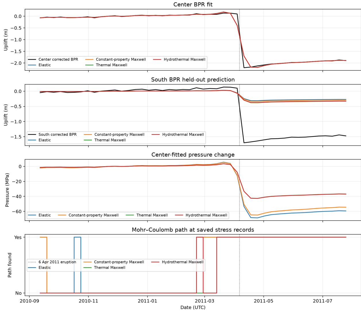
Figure 26: Four rheology fits to the MGDS NeMO 2010–11 Center DriftCorrSpot1Dep channel, corrected for predicted tide and MPR drift, with the tide-corrected 2009–11 South Spot1DetidedDepth channel held out. Non-tidal ocean variability remains. The Center fit includes eruption deflation and subsequent observations. Sources: MGDS IEDA/322282, Chadwick et al. (2023), CC BY-NC-SA 3.0.
