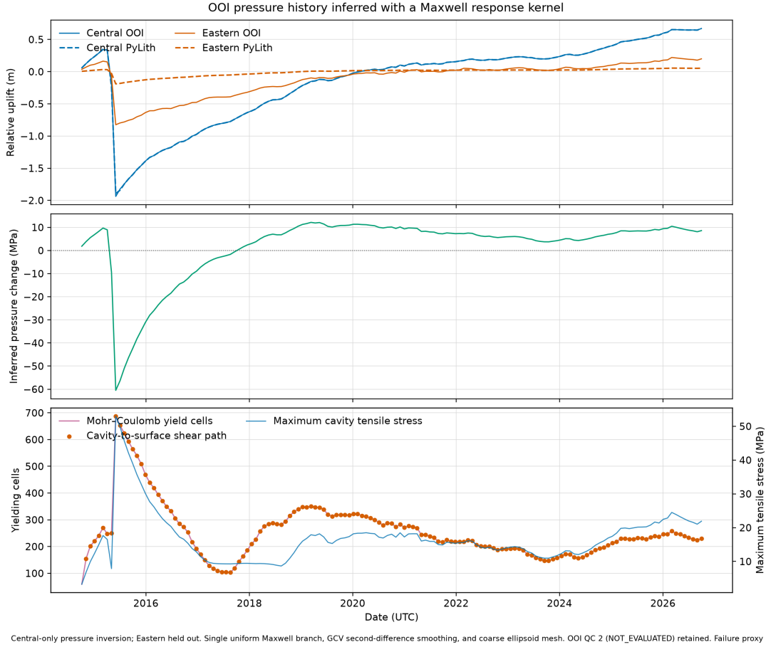
Figure 20: OOI Central pressure inversion with a one-branch Maxwell response kernel. Central is fitted and Eastern is held out; dashed curves show the direct PyLith history. The plot includes the inferred pressure and provisional failure diagnostics. Generated by make ooi-maxwell-pressure-inversion from independent OOI records. The smoothness prior, pressure scale, and nonconverged mesh remain provisional.
