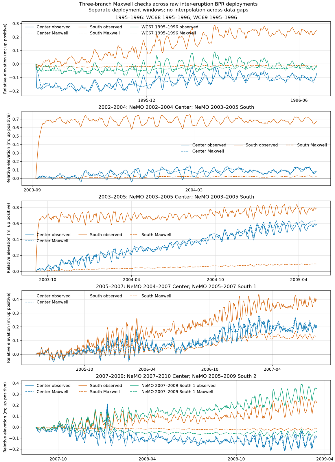
Figure 14: Three-branch Maxwell checks for raw Center/South deployment overlaps from 1995 through 2009. WC67 is held out in 1995–96 and NeMO South 1 in 2007–09. Each pair is independently zeroed; gaps are not interpolated. Generated by make reproduce .
