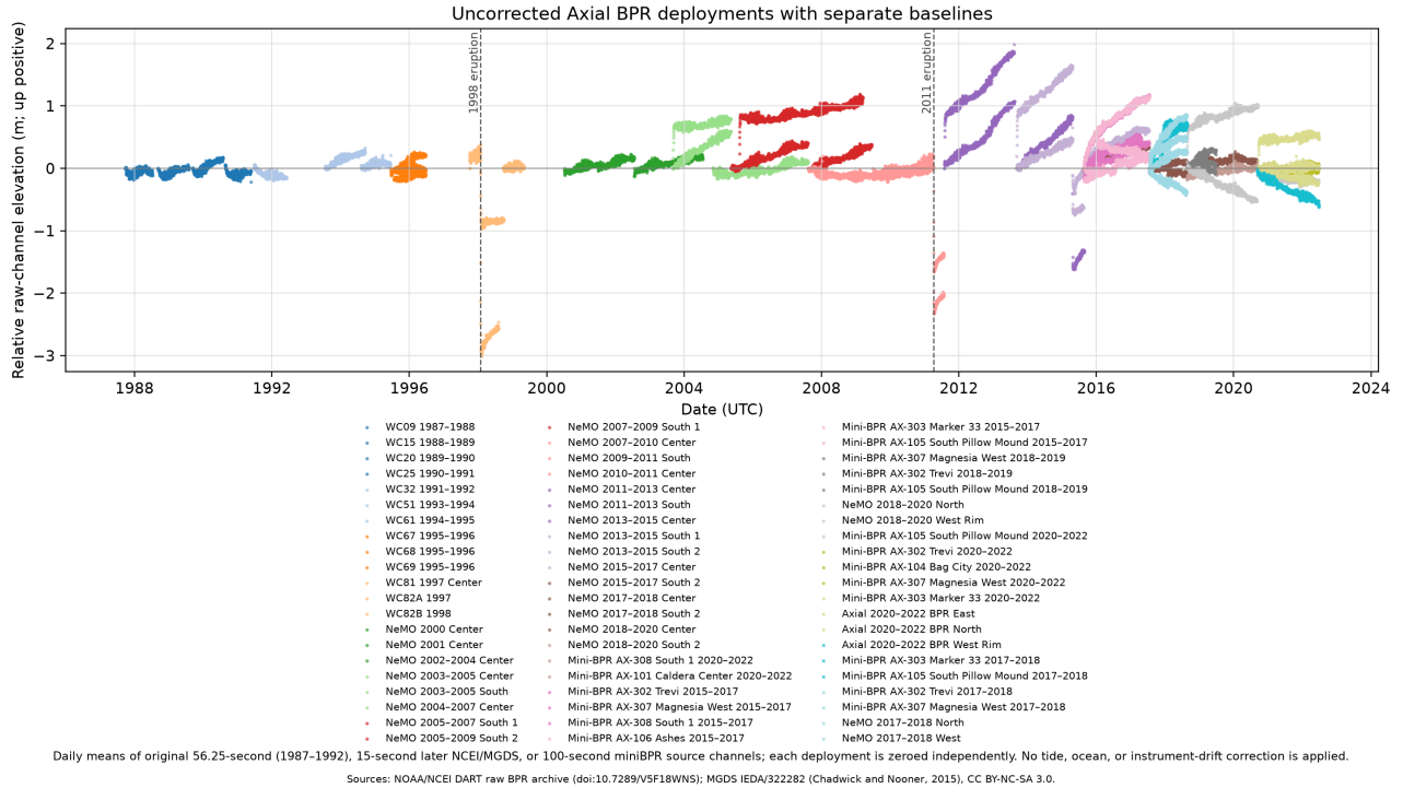
Figure 8: Separate-baseline daily means of original raw non-OOI BPR channels from 1987 through 2022. The plot shows intermittent deployment coverage; each segment is zeroed independently and remains uncorrected for tides, ocean variability, and instrument drift. Generated by make bpr-historical-check . Sources: NOAA/NCEI DART raw BPR archive (doi:10.7289/V5F18WNS) and MGDS IEDA/322282 (Chadwick and Nooner, 2015). MGDS-derived values are distributed under CC BY-NC-SA 3.0.
