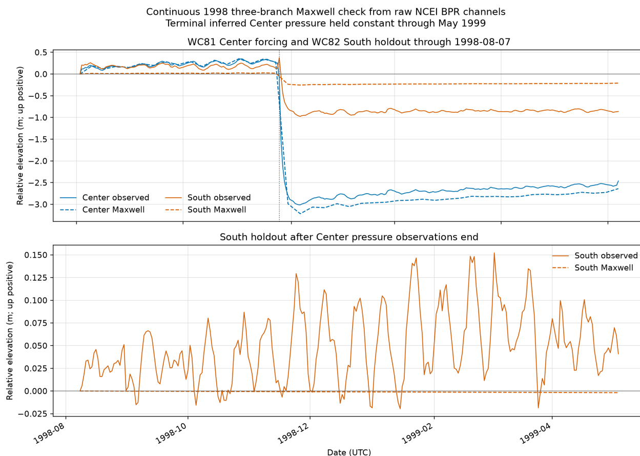
Figure 12: Continuous 1998 three-branch Maxwell check using only original NCEI WC81 Center and WC82 South absolute-pressure channels. The upper panel compares Center forcing and the event South holdout through 7 August 1998; the lower panel checks the South station through 4 May 1999 after Center pressure observations end. The two WC82 South files are aligned from their eight-day raw overlap. Terminal inferred Center pressure is held constant for 270 days. Synthetic branch parameters, raw ocean variability, and nonconverged compliance limit interpretation. Source: NCEI DART raw BPR archive, doi:10.7289/V5F18WNS. Generated by make historical-generalized-maxwell-1998-continuous-check .
