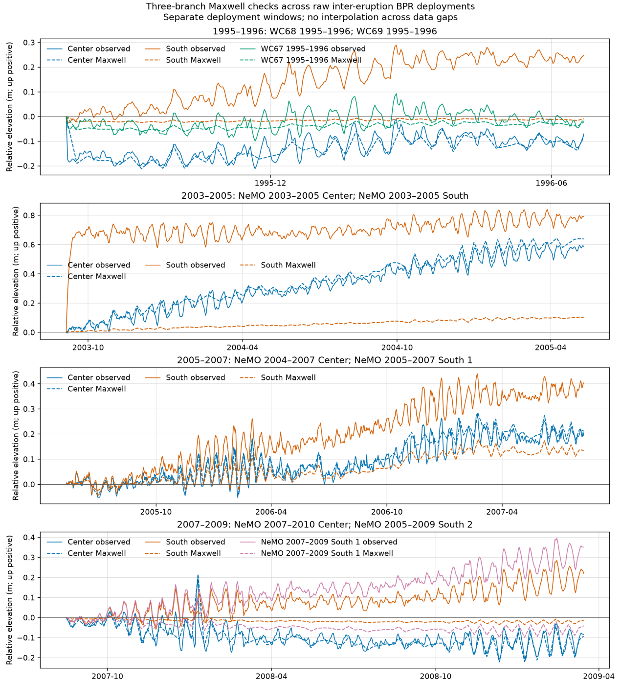
Figure 9: Three-branch Maxwell checks for raw Center/South deployment overlaps from 1995 through 2009. WC67 is held out in 1995–96 and NeMO South 1 in 2007–09. Each pair is independently zeroed; gaps are not interpolated. Generated by make reproduce .
