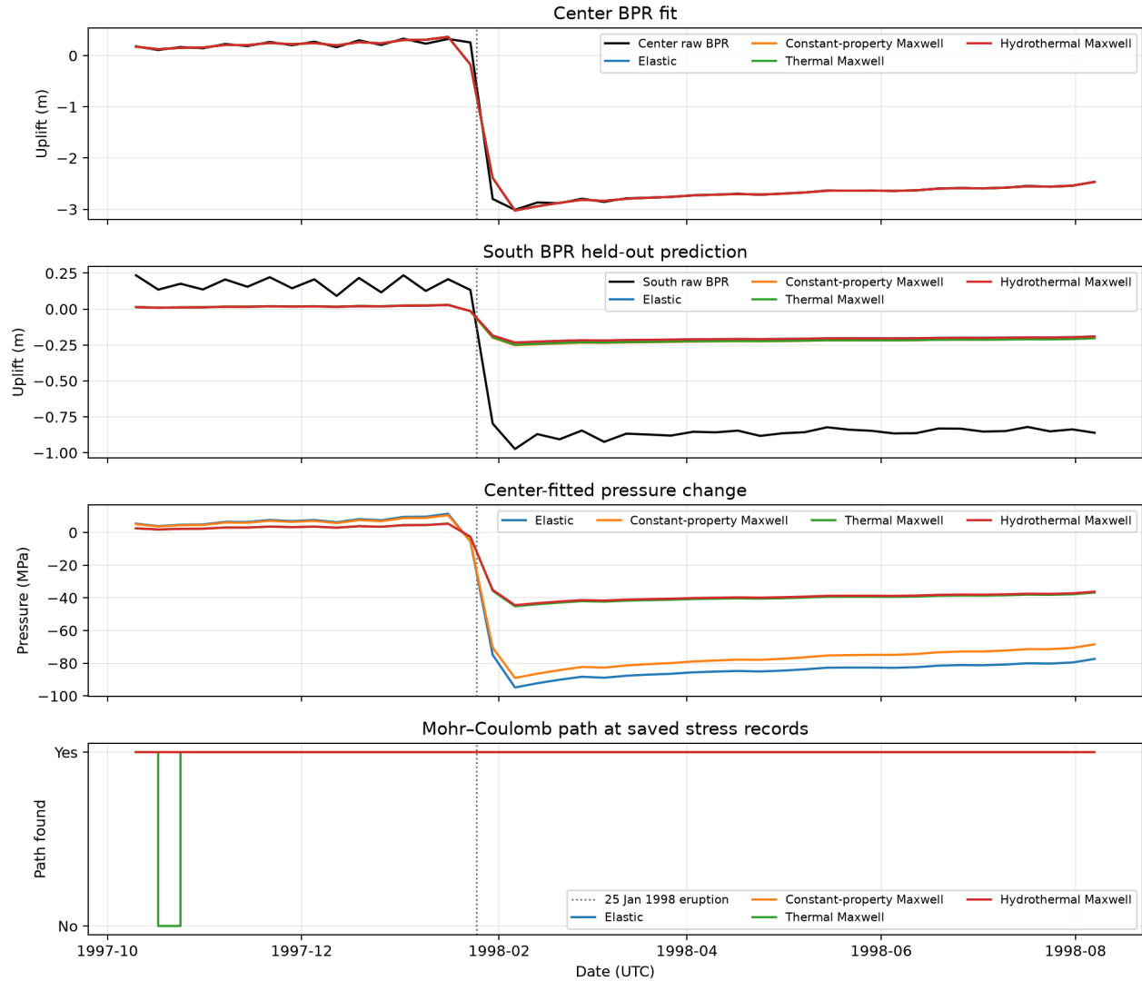
Figure 17: Four pressure calibrations against original raw NCEI WC81 Center data, with WC82A South held out and provisional connected-path states shown at saved stress records. The dotted line marks the observed 25 January 1998 eruption. Each pressure history is fitted independently, and Center includes the eruption deflation and later records. Synthetic branch parameters, the nonconverged mesh, and unresolved failure assumptions make this a retrospective diagnostic. No MGDS Fox duplicate or Cabaniss-associated data products were used. Generated by make historical-four-case-bpr-calibration .
