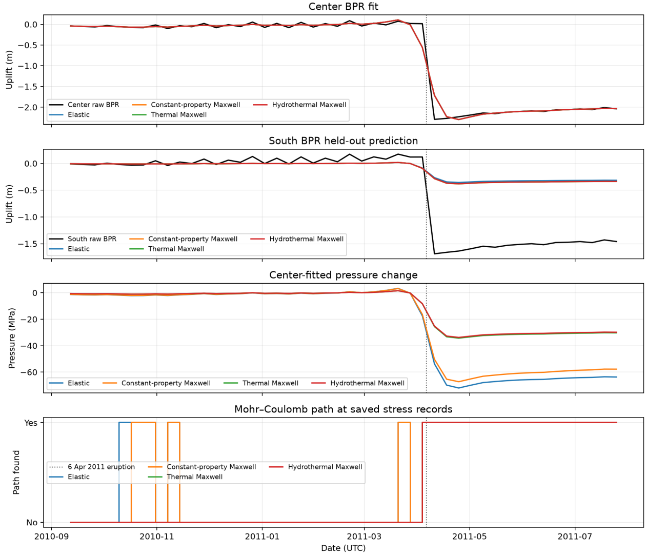
Figure 18: Four pressure calibrations against original raw NeMO Center BPR data, with NeMO South held out and provisional connected-path states shown at saved stress records. Dotted vertical lines mark the observed 6 April 2011 eruption. Each pressure history is fitted independently; the Center input includes the eruption deflation and subsequent data. Synthetic branch parameters, the nonconverged mesh, and unresolved failure assumptions make this a retrospective diagnostic. Generated by make historical-four-case-bpr-calibration . Sources are original MGDS IEDA/322282 RawDep/Depth channels (William Chadwick, Scott Nooner, and MGDS; CC BY-NC-SA 3.0).
