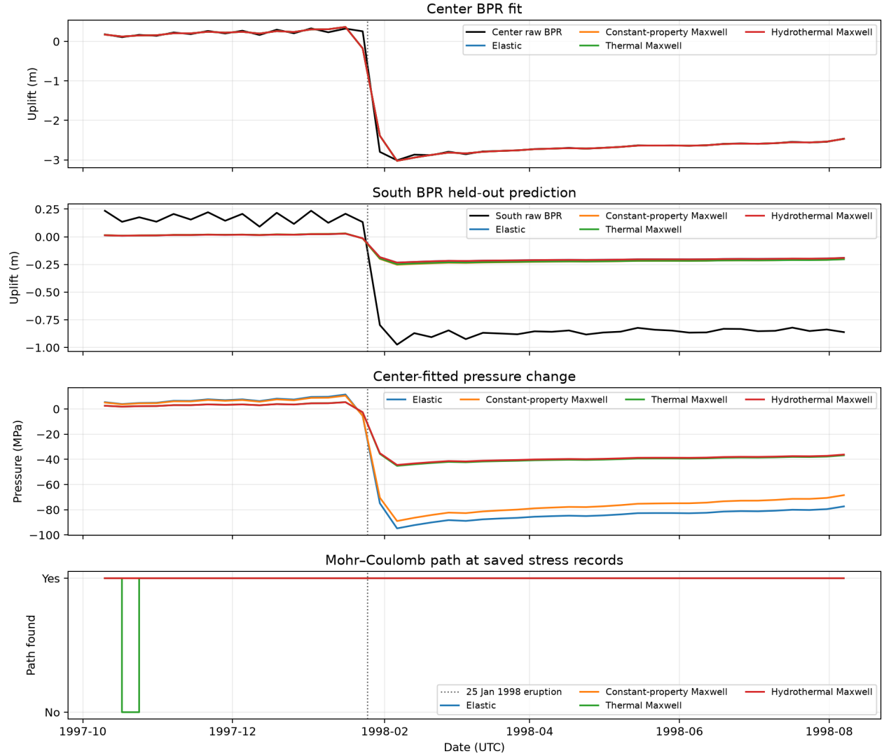
Figure 16: Four pressure calibrations against original raw NCEI WC81 Center data, with WC82A South held out and provisional connected-path states shown at saved stress records. The dotted line marks the observed 25 January 1998 eruption. Each pressure history is fitted independently, and Center includes the eruption deflation and later records. Synthetic branch parameters, the nonconverged mesh, and unresolved failure assumptions make this a retrospective diagnostic. No MGDS Fox duplicate or Cabaniss-associated data products were used. Generated by make historical-four-case-bpr-calibration .
