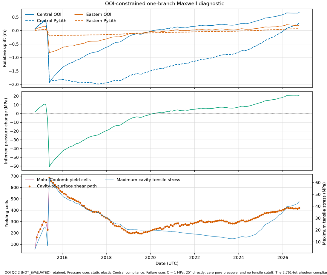
Figure 10: OOI-constrained one-branch Maxwell diagnostic. The panels compare OOI and modeled uplift, static-fit pressure, and stress-derived failure indicators. Generated by make ooi-maxwell-history-plot . Quality code 2 is retained; pressure uses static compliance; the mesh and failure assumptions remain provisional.
