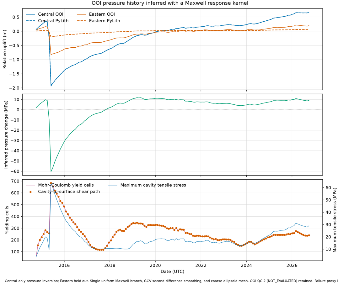
Figure 14: OOI Central pressure inversion with a one-branch Maxwell response kernel. Central is fitted and Eastern is held out; dashed curves show the direct PyLith history. The plot includes the inferred pressure and provisional failure diagnostics. Generated by make ooi-maxwell-pressure-inversion from independent OOI records. The smoothness prior, pressure scale, and nonconverged mesh remain provisional.
